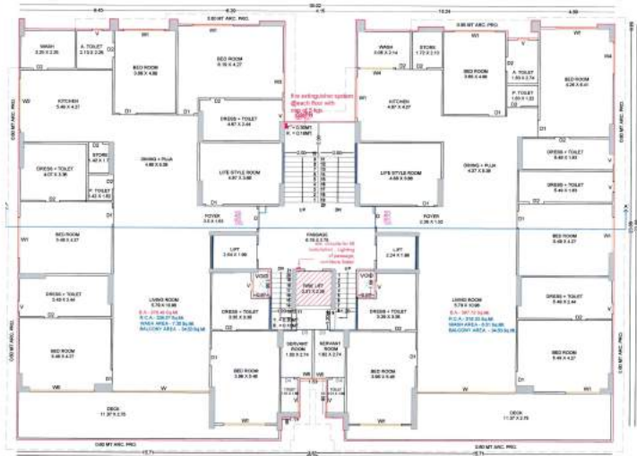
TYPICAL FL. (1st, 4th, 8th &amp; 12th) PLAN
