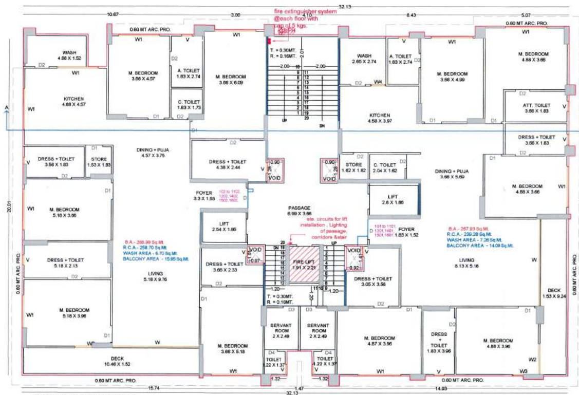
TYPICAL FL. (1 ST TO 15 TH) PLAN
