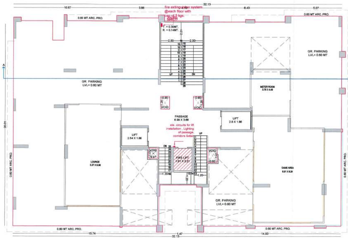
GROUND FL. PLAN
