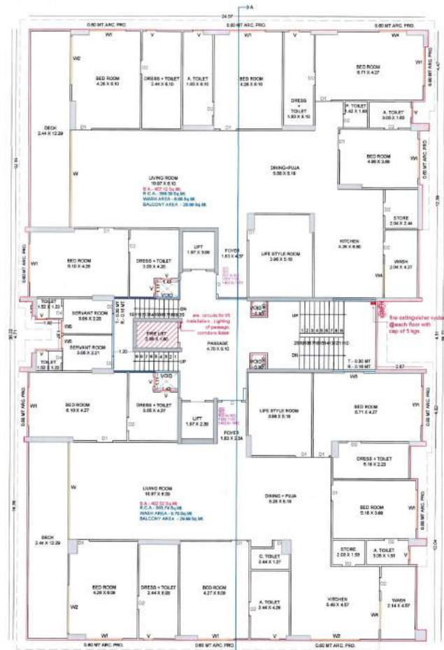
TYPICAL FL. (2nd, 3rd, 5th to 8th, 10th, 11B, 12B to 13B) PLAN
