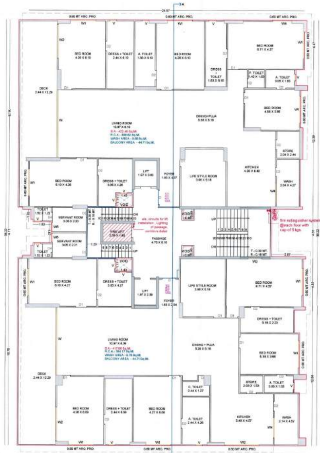
TYPICAL FL. (11, 11A, 11B &amp; 12B) PLAN
