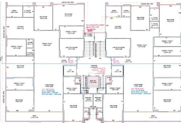
TYPICAL FL. (2nd, 3rd, 5th, 6th, 10th, 11th, 13th, &amp; 14th) PLAN
