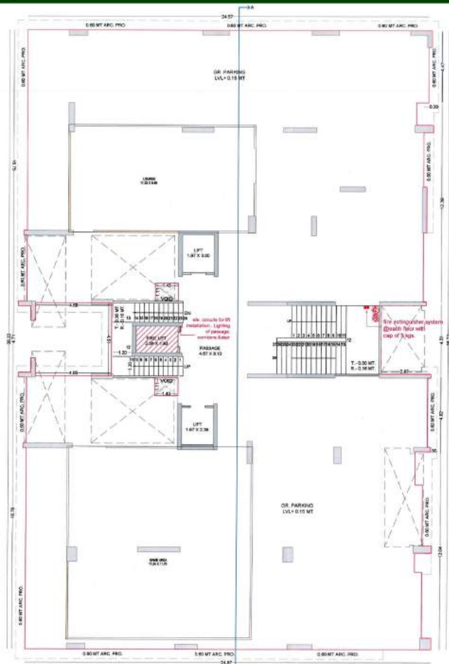
BUILDING J GROUND FL. PLAN
