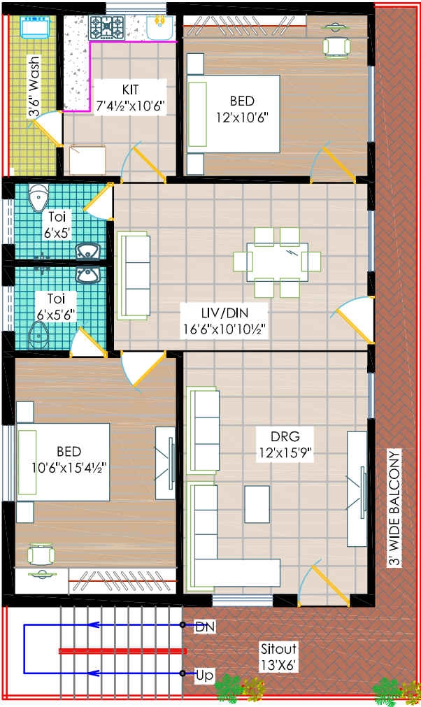
FIRST FLOOR PLAN 1215 Sft
