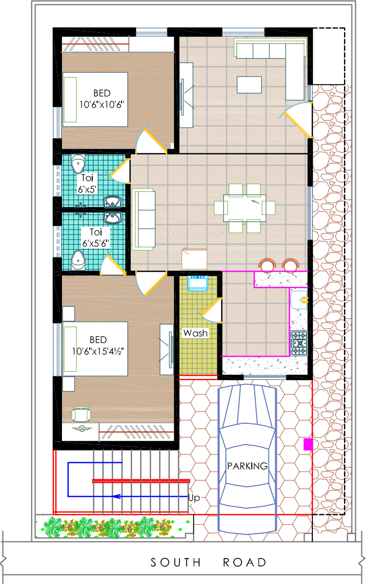
GROUND FLOOR PLAN 1080 Sft
