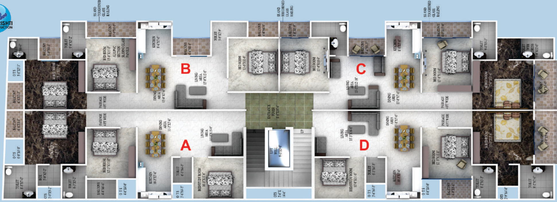
TYPICAL FLOOR PLAN OF 'SRISHTI RESIDENCY'
