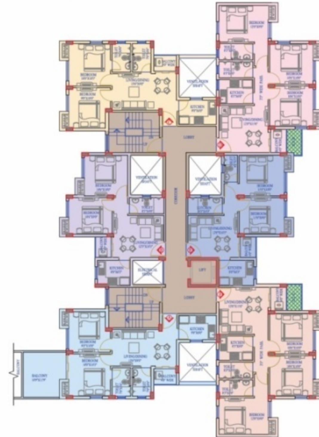
Block 4 | 2 nd floor plan
