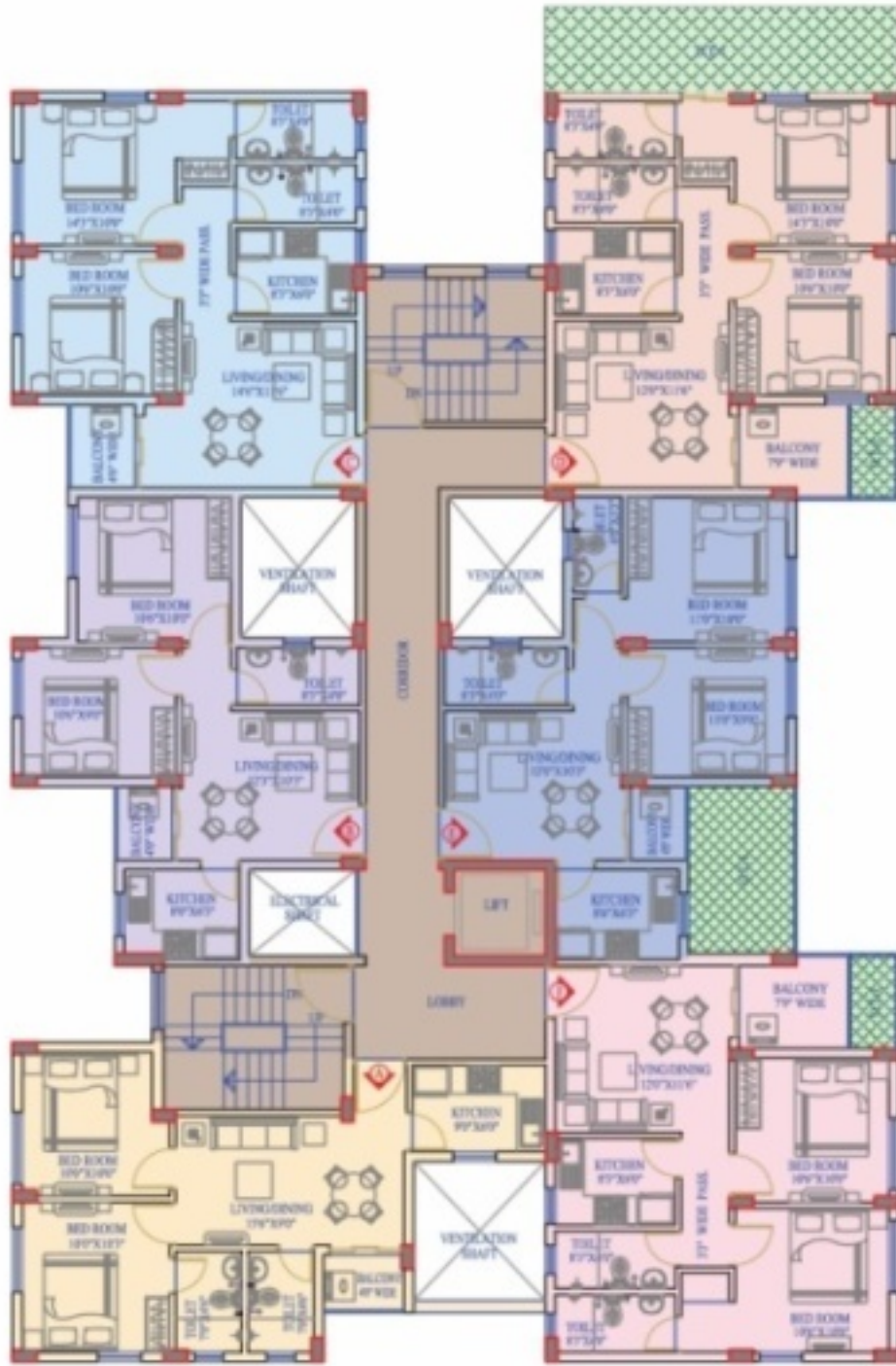
Block 5 | 1 st floor plan
