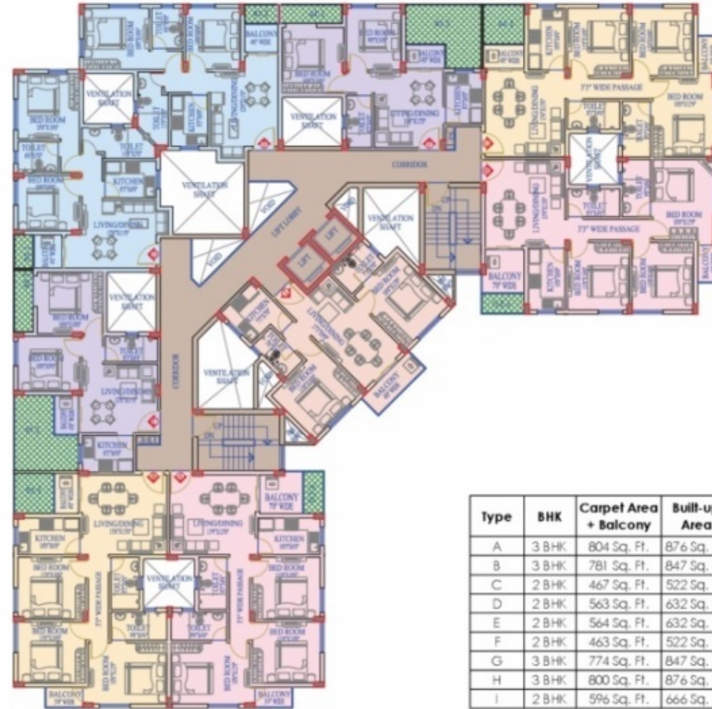
Block 2 | 1 st floor plan
