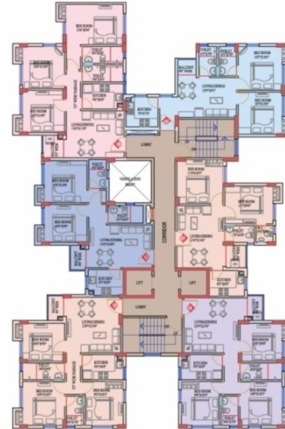
Block 12 | Typical floor plan
