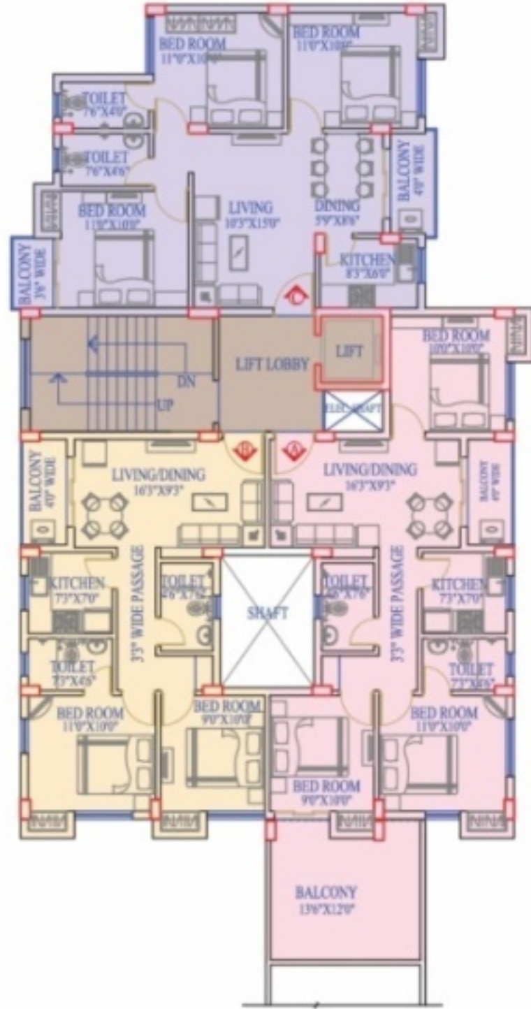
Block 6 | 2 nd floor plan
