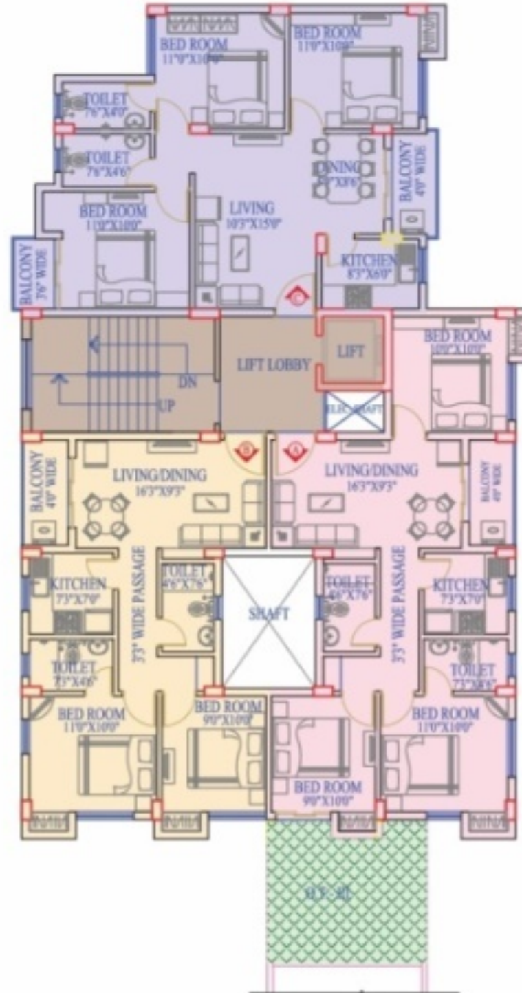
Block 6 | Typical floor plan
