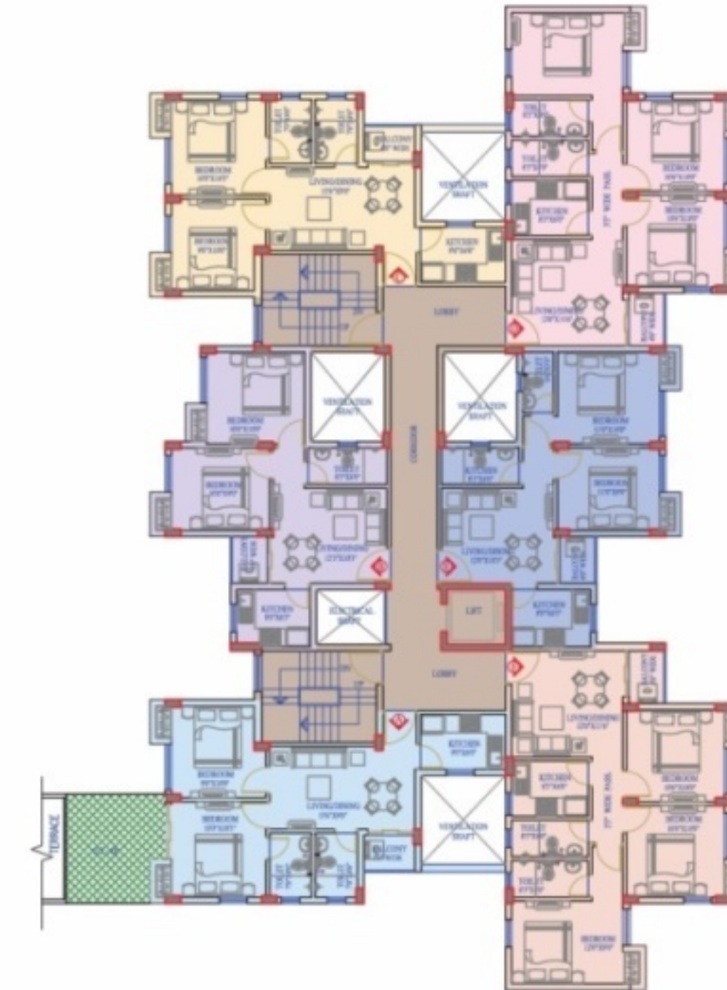
Block 4 | Typical floor plan
