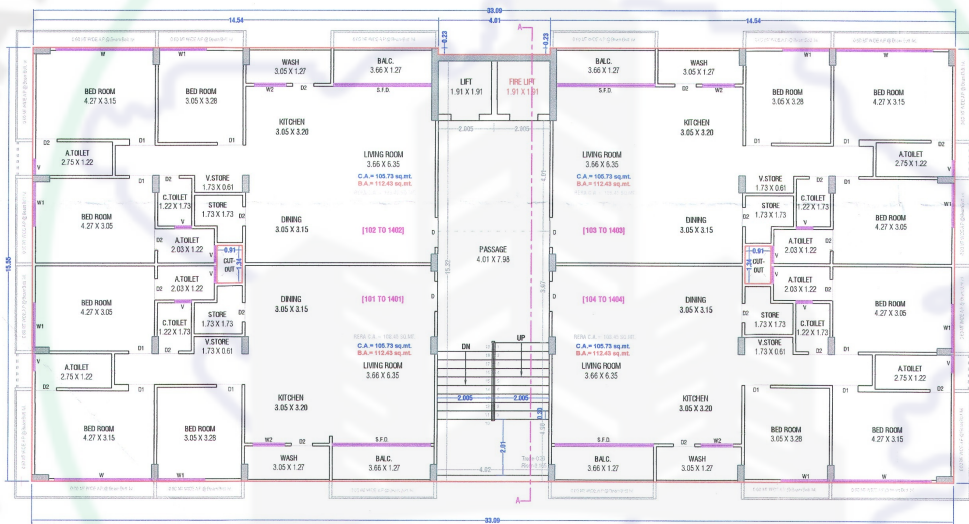
TYPICAL FLOOR PLAN (1st to 14th. FLOOR)
