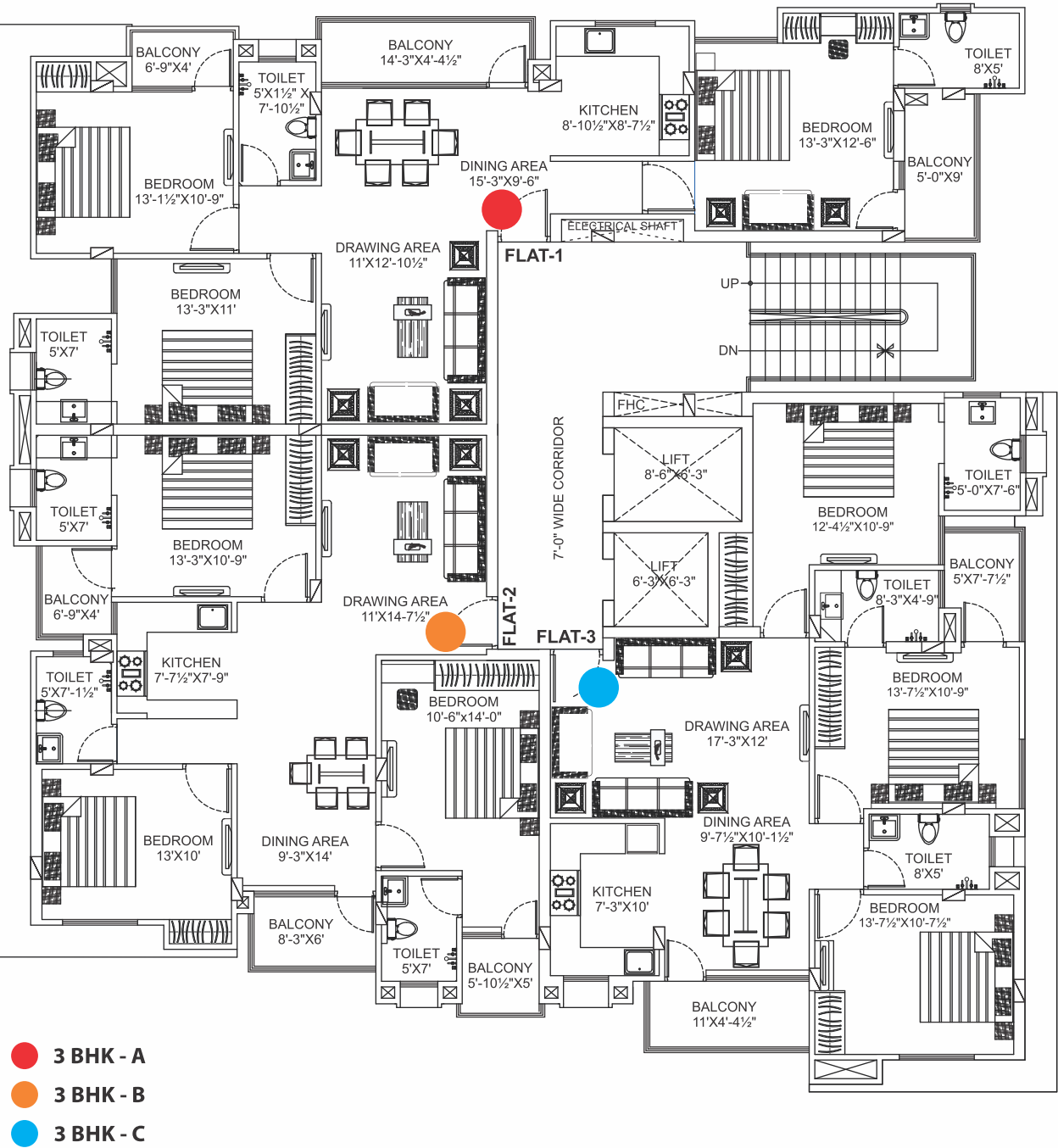
1st - 8th Floor Plan
