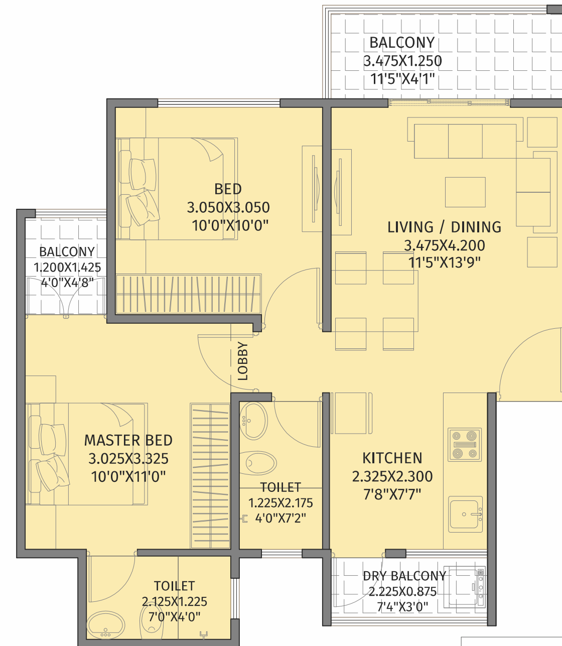
Floor Plan 2 BHK (Type 1)
