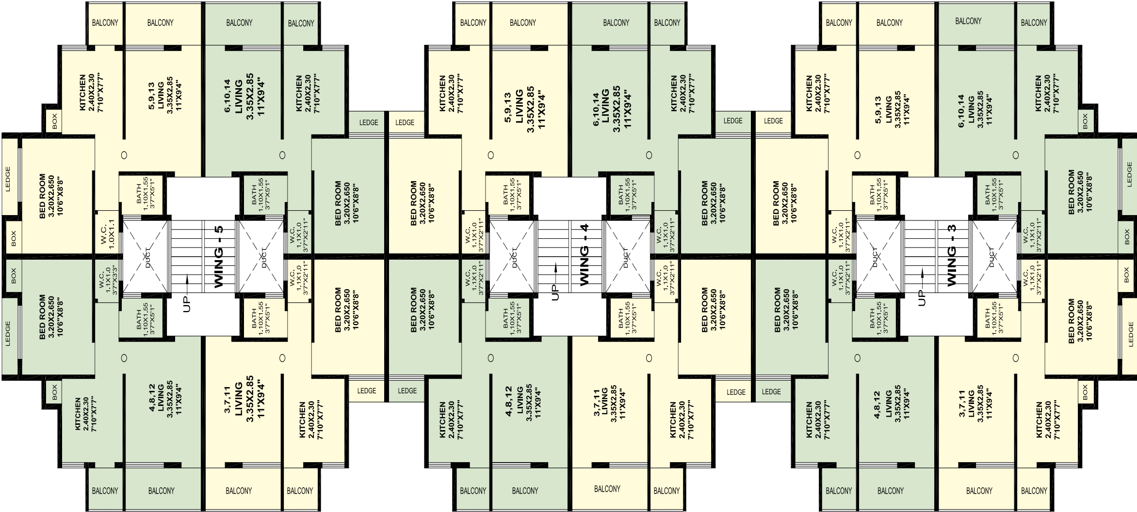
Typical Stilt First & First Floor Plan; Stilt Second & Second Floor Plan; Stilt Third & Third Floor Plan
