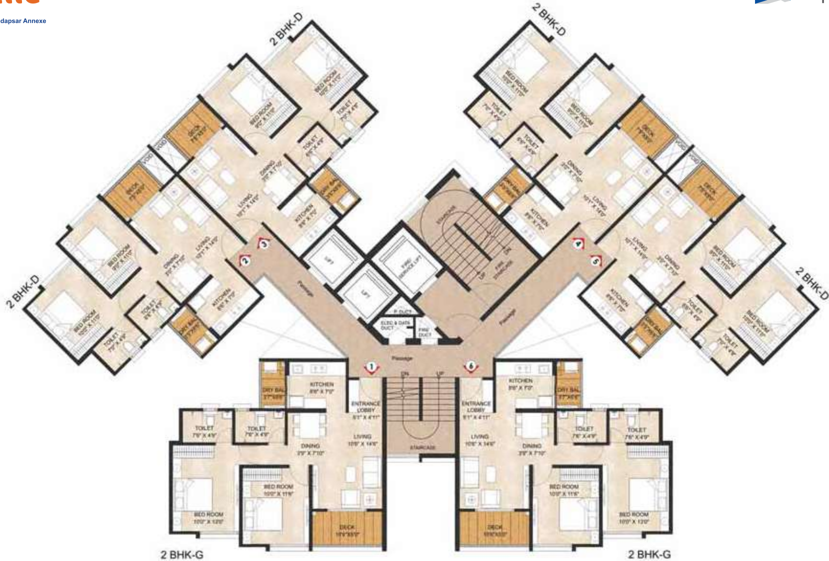
TP2-TYPICAL FLOOR PLAN - TOWER-8
