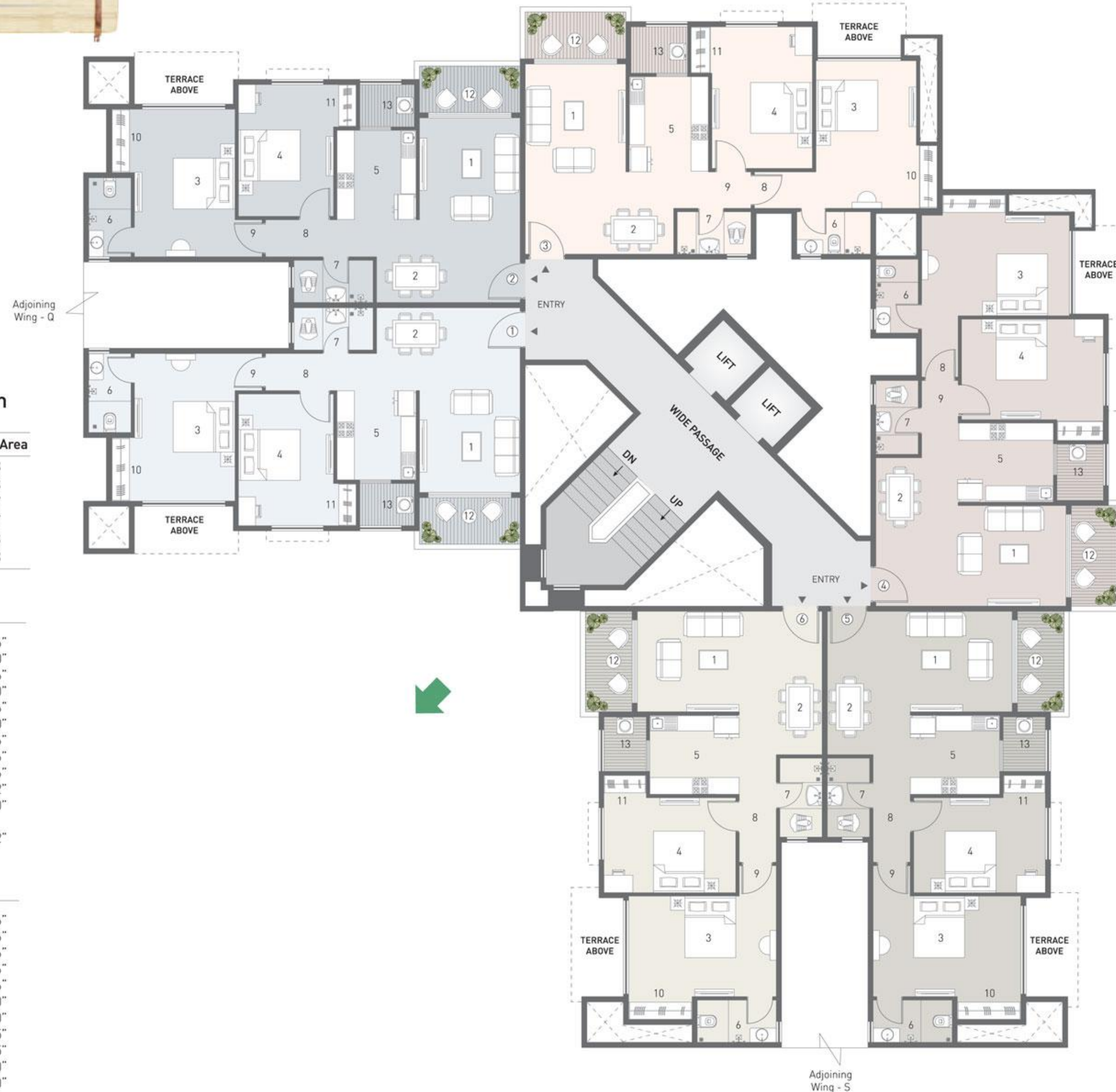
2nd, 4th & 6th floor plan
