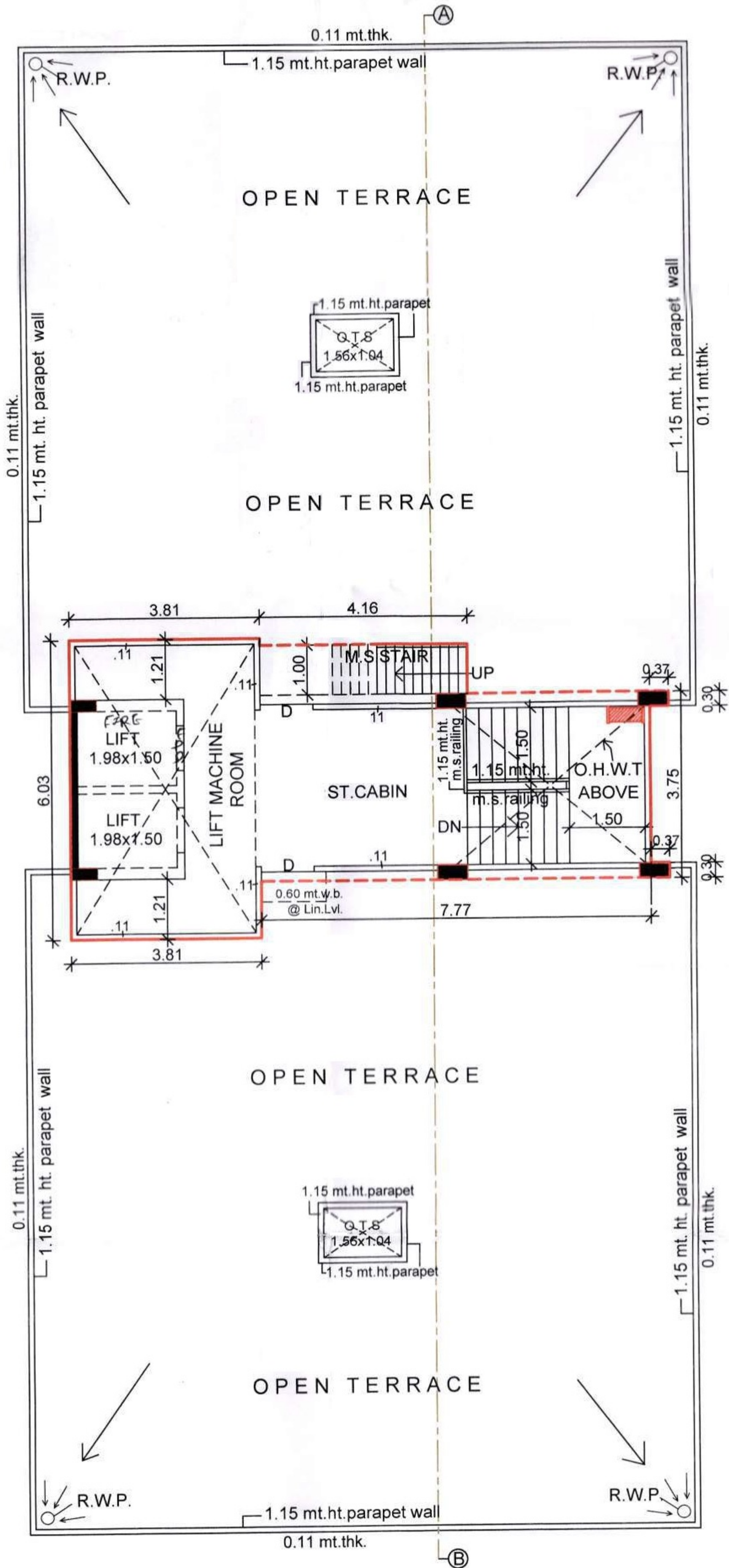
STAIR CABIN , LIFT MACHINE ROOM & OPEN TERRACE PLAN
