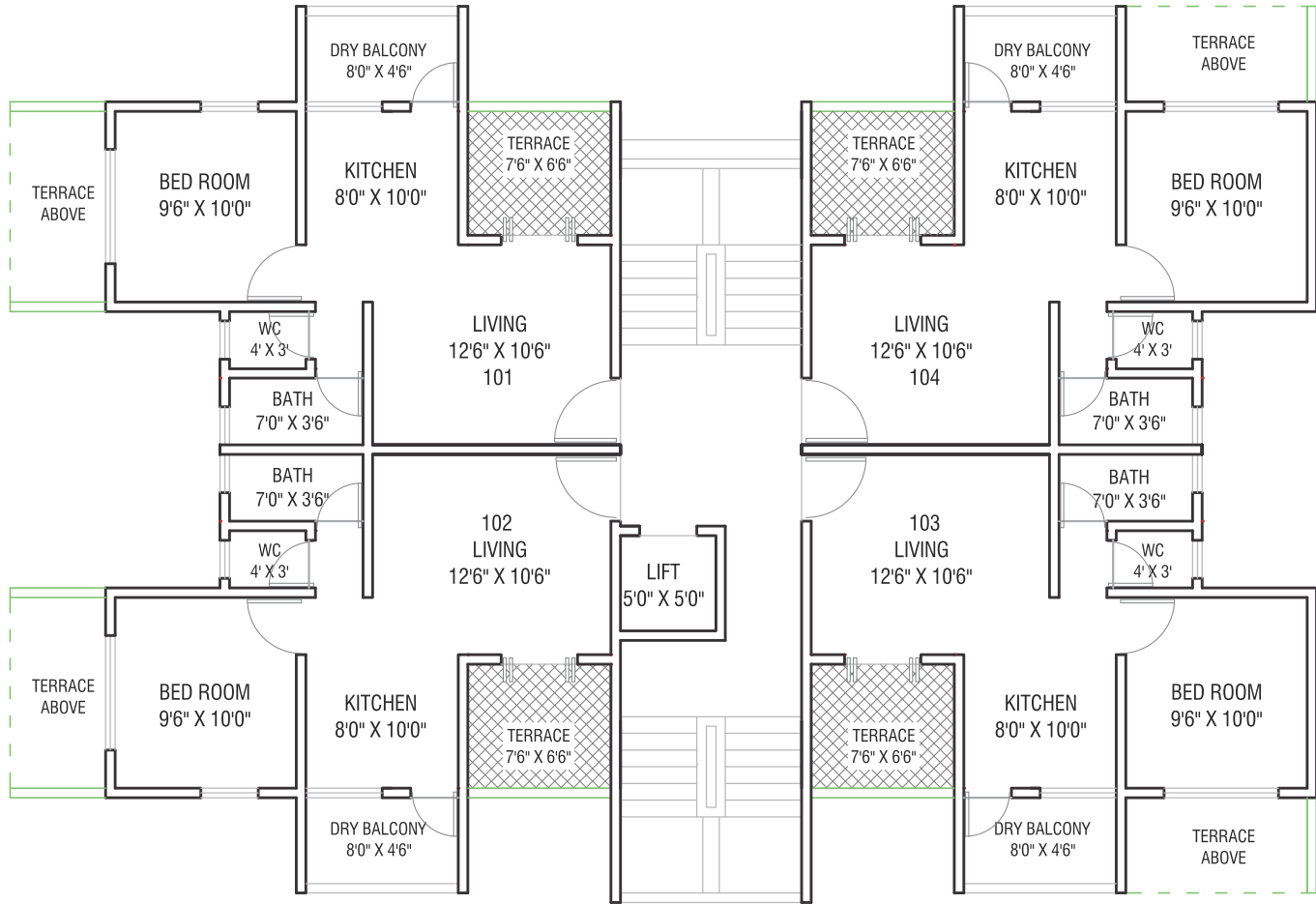
TYPICAL FLOOR PLAN (1ST, 3RD, 5TH, FLOOR)
