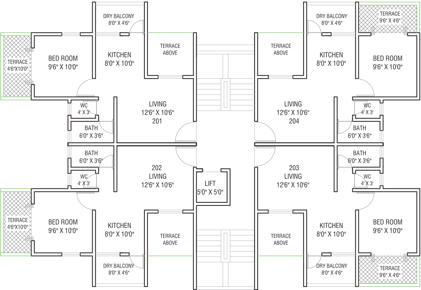
TYPICAL FLOOR PLAN (2ND, 4TH, 6TH FLOOR)
