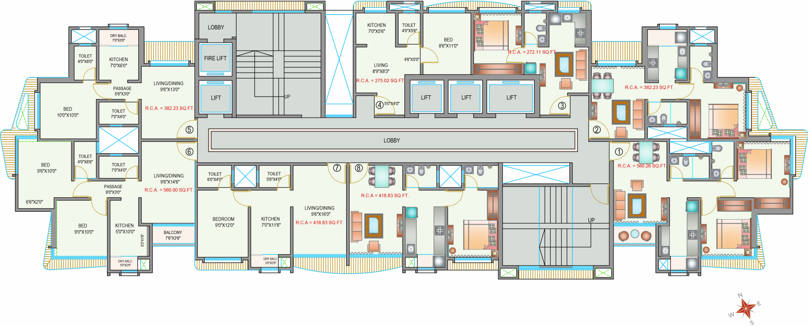
Typical Floor Plan
