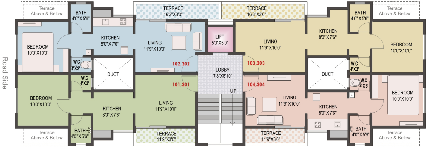
1 st & 3 rd Floor Plan
