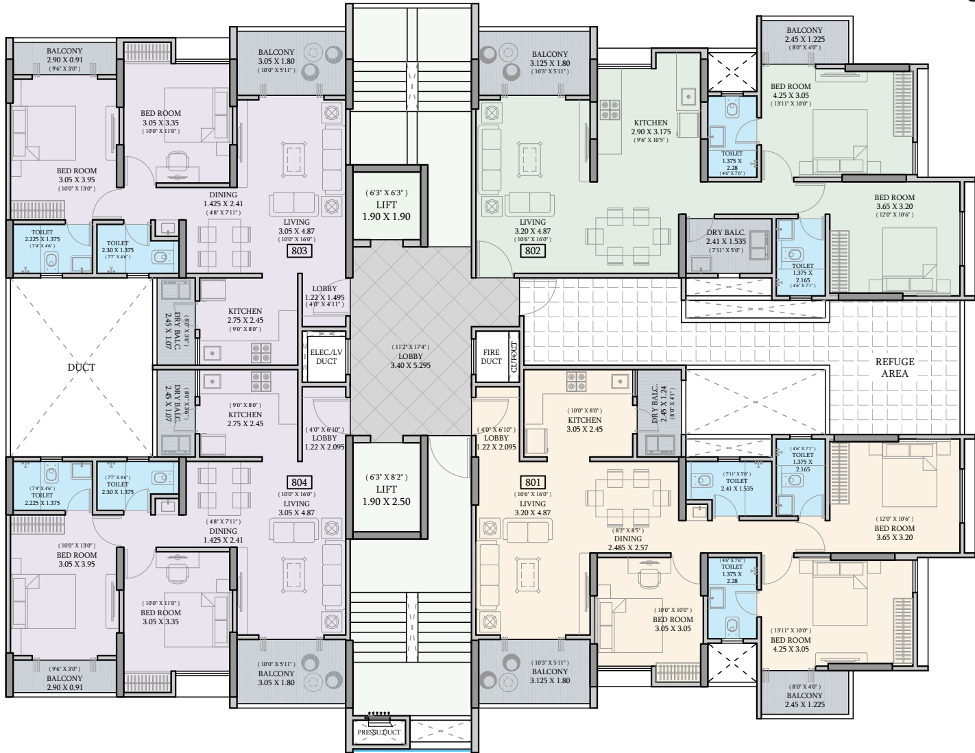
AREA STATEMENT (WING - A7) (REFUGE FLOOR)
