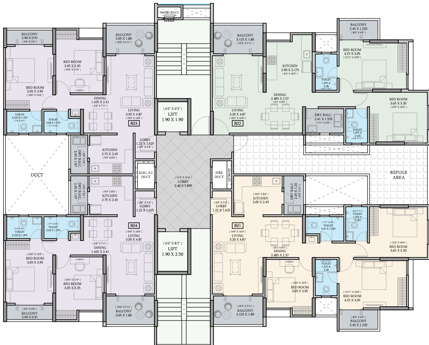
AREA STATEMENT (WING - A6) (REFUGE FLOOR)
