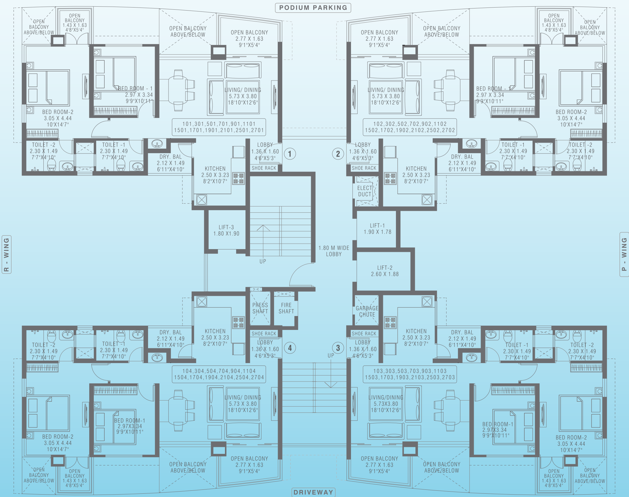
1 st , 3 rd , 5 th , 7 th , 9 th , 11 th , 15 th , 17 th , 19 th , 21 st , 25 th , 27 th FLOOR PLAN
