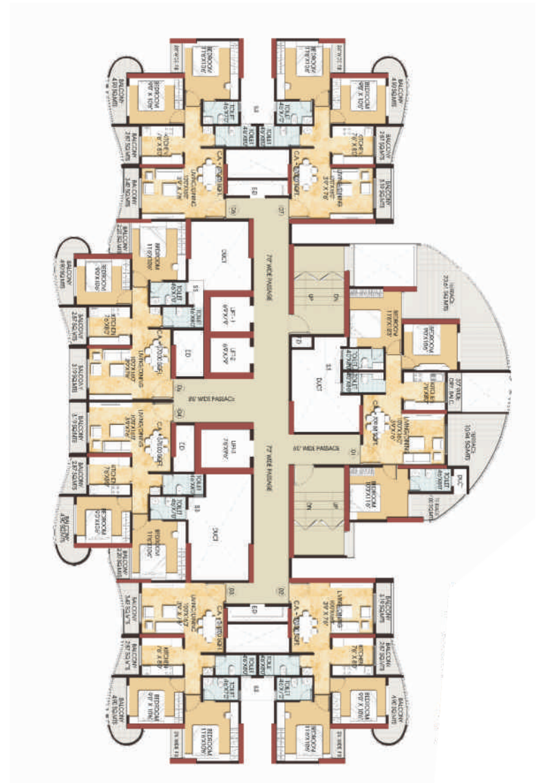
TYPICAL 34TH FLOOR
