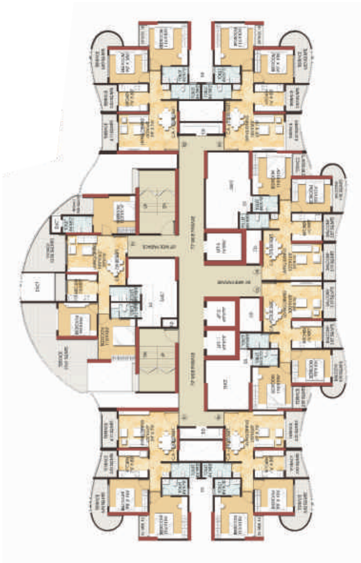
TYPICAL 11TH & 36TH FLOOR
