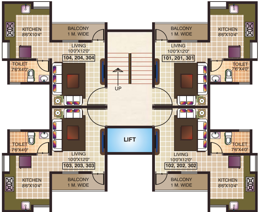
TYPICAL FLOOR PLANS OF WING : F, G & H
