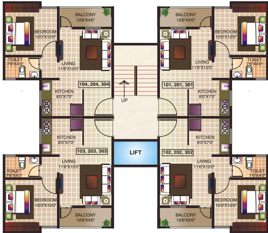
TYPICAL FLOOR PLANS OF WING : D
