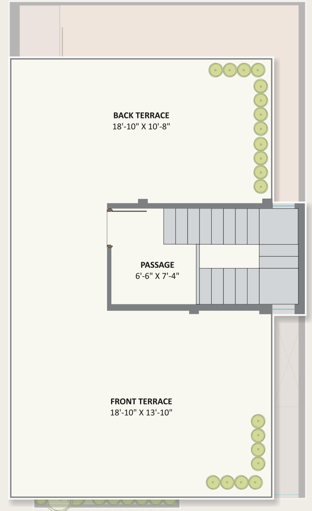
Terrace Floor Built-UP Area - 141.5 Sq.Ft. Carpet Area - 105 Sq.Ft.
