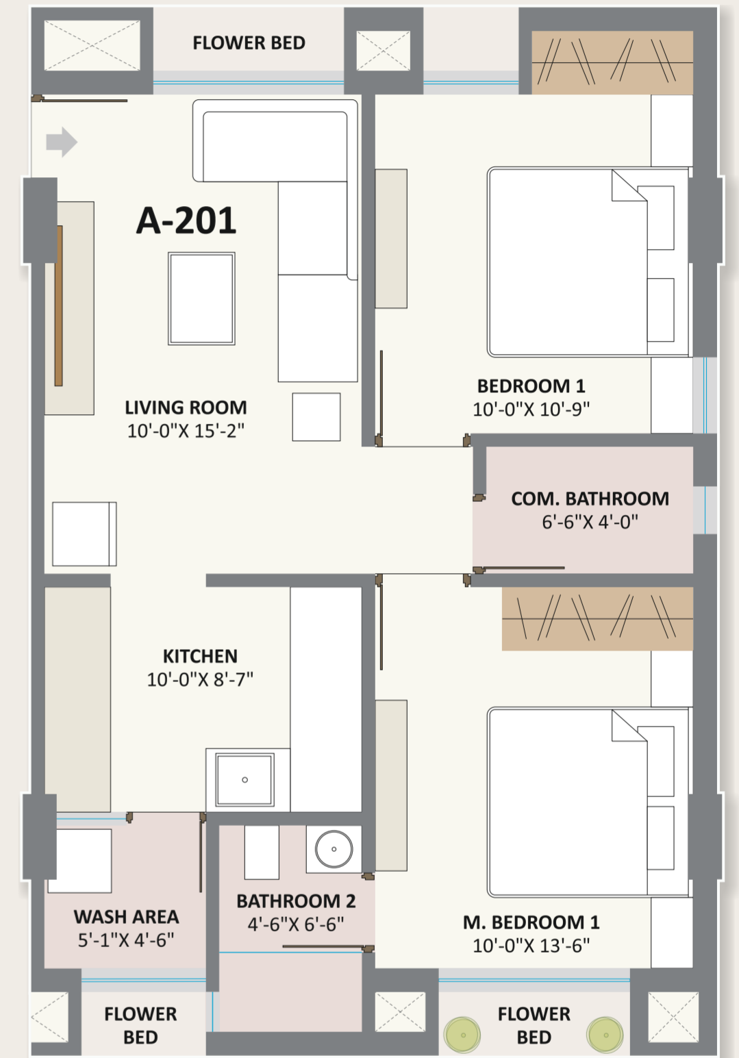
Type A ( 2 BHK ) Built-UP Area - 626 Sq.Ft. Carpet Area - 558 Sq.Ft.
