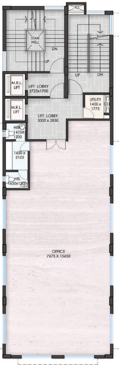
2nd Floor Plan of Block 5
