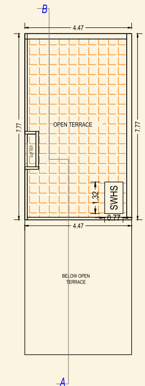
TERRACE FLOOR PLAN (SCALE 1:100)
