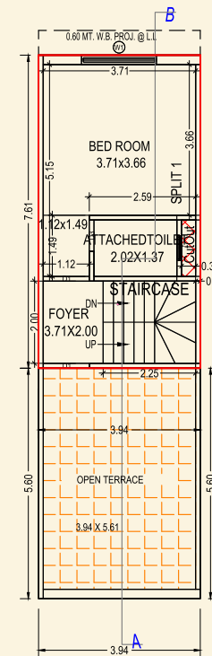
SECOND FLOOR PLAN (Proposed) (SCALE 1:100)
