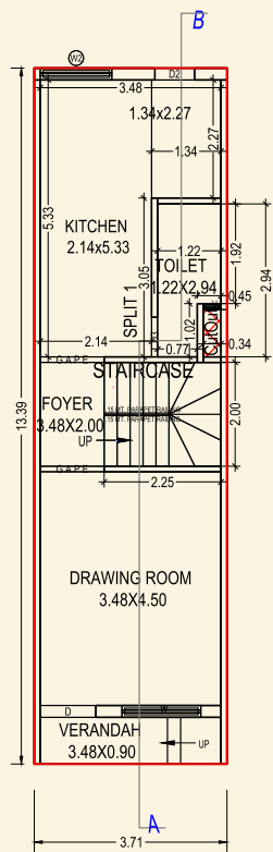
GROUND FLOOR PLAN (Proposed)
