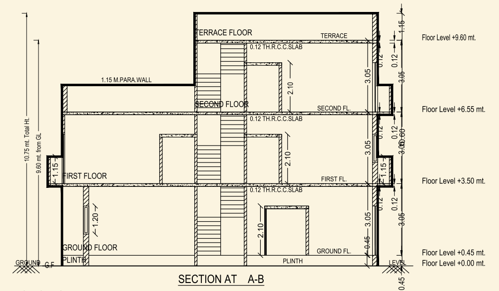
SECTION SECTION AT A-B
