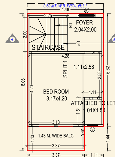
FIRST FLOOR PLAN (Proposed) (SCALE 1:100)
