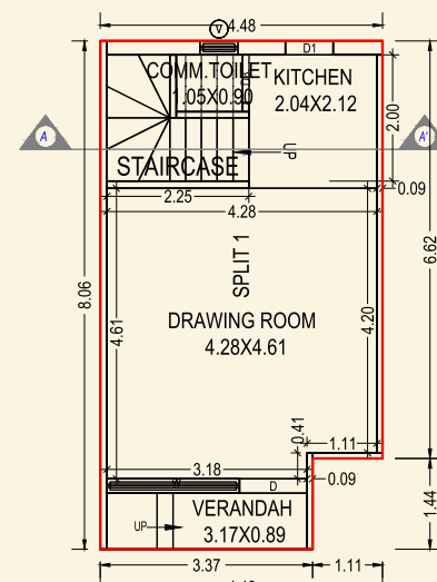
GROUND FLOOR PLAN (Proposed) (SCALE 1:100)
