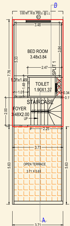
SECOND FLOOR PLAN (Proposed)
