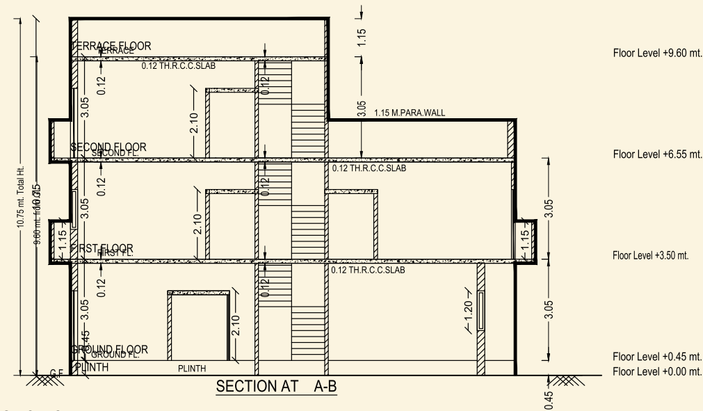
SECTION
