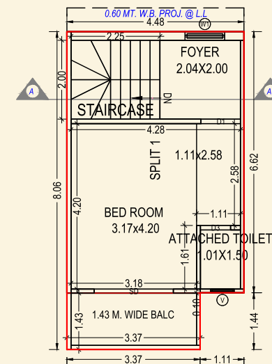
SECOND FLOOR PLAN (Proposed) (SCALE 1:100)
