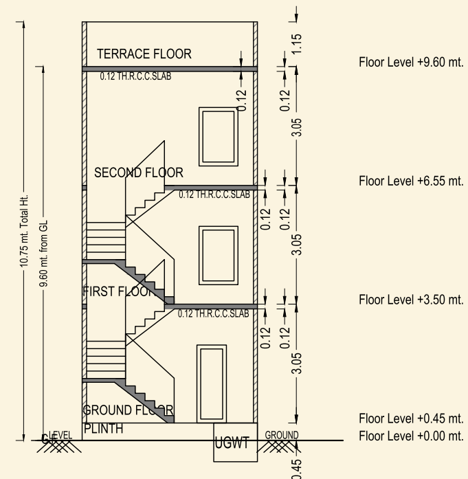
SECTION
