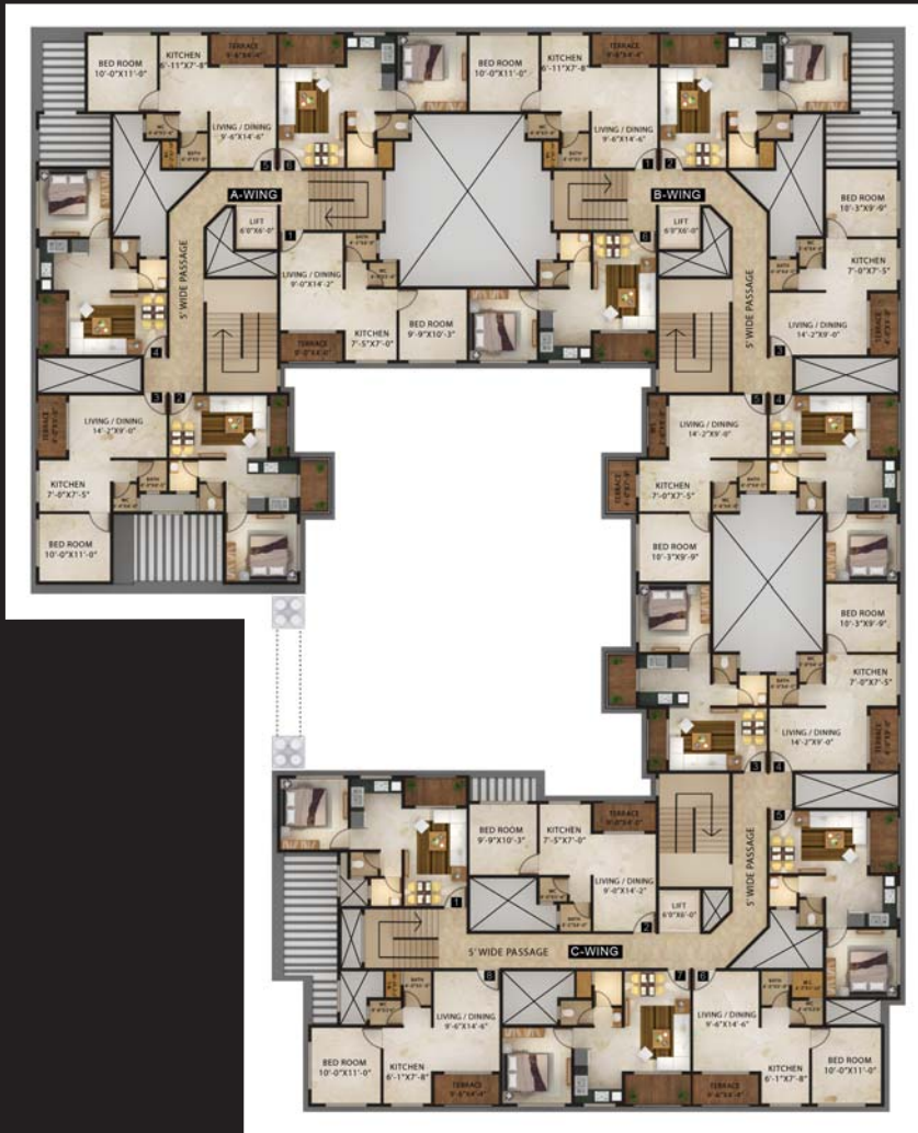
Building 4: First floor plan
