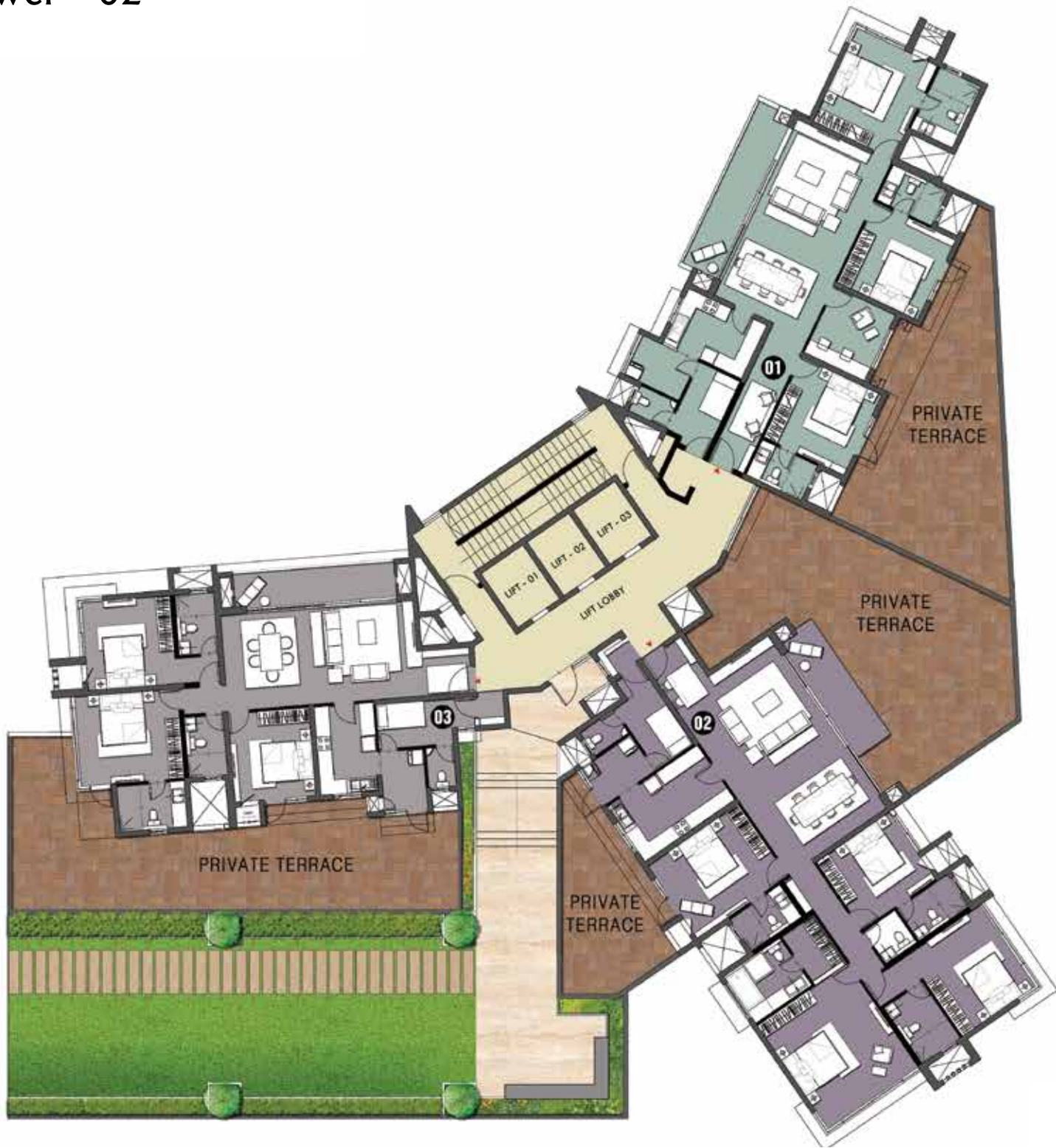
2 nd Floor Plan Tower - 02
