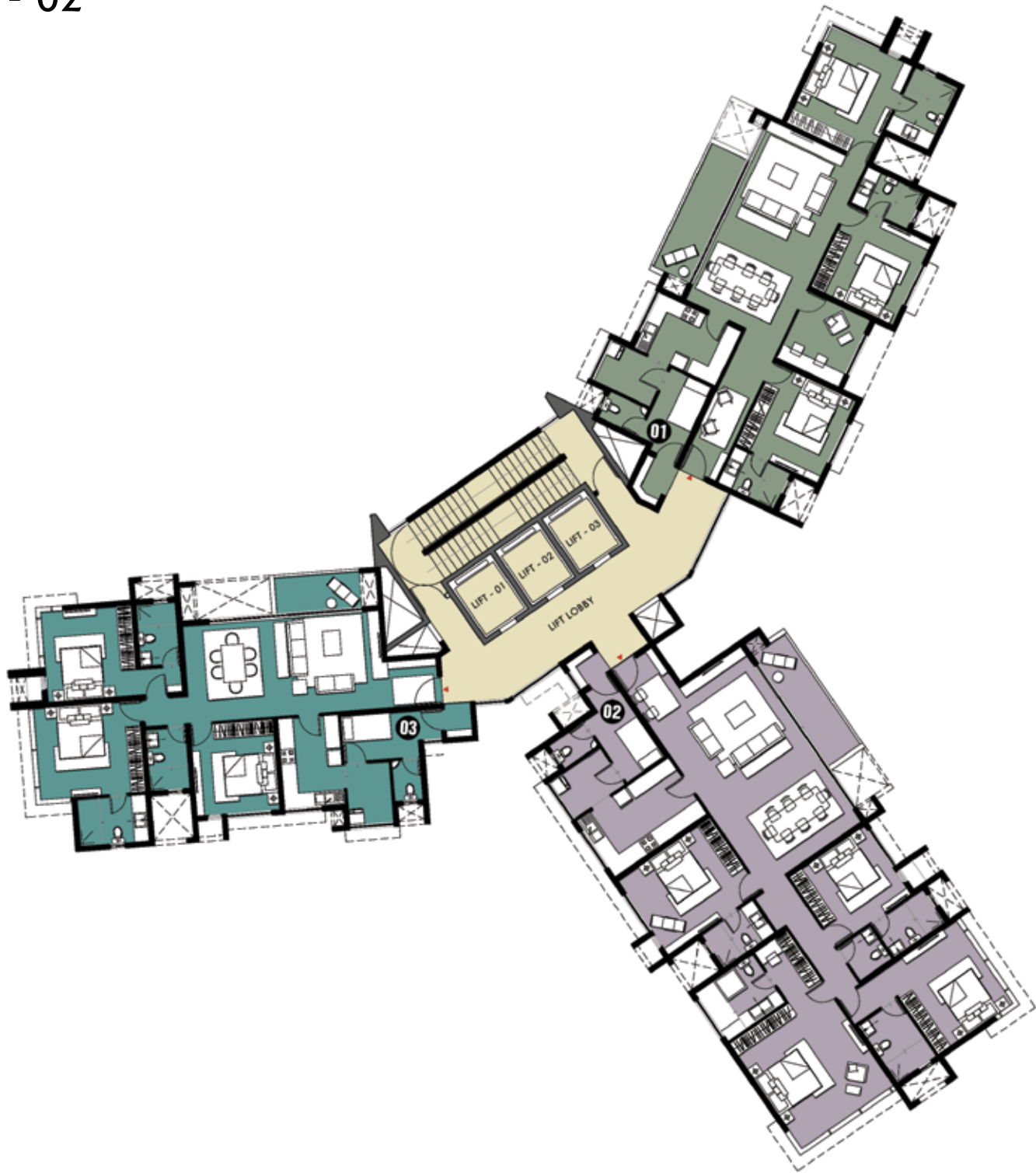
04 th , 06 th , 08 th , 10 th , 12 th , 14 th , 16 th , 18 th , 20 th , 22 nd , 24 th Floor Plan Tower - 02
