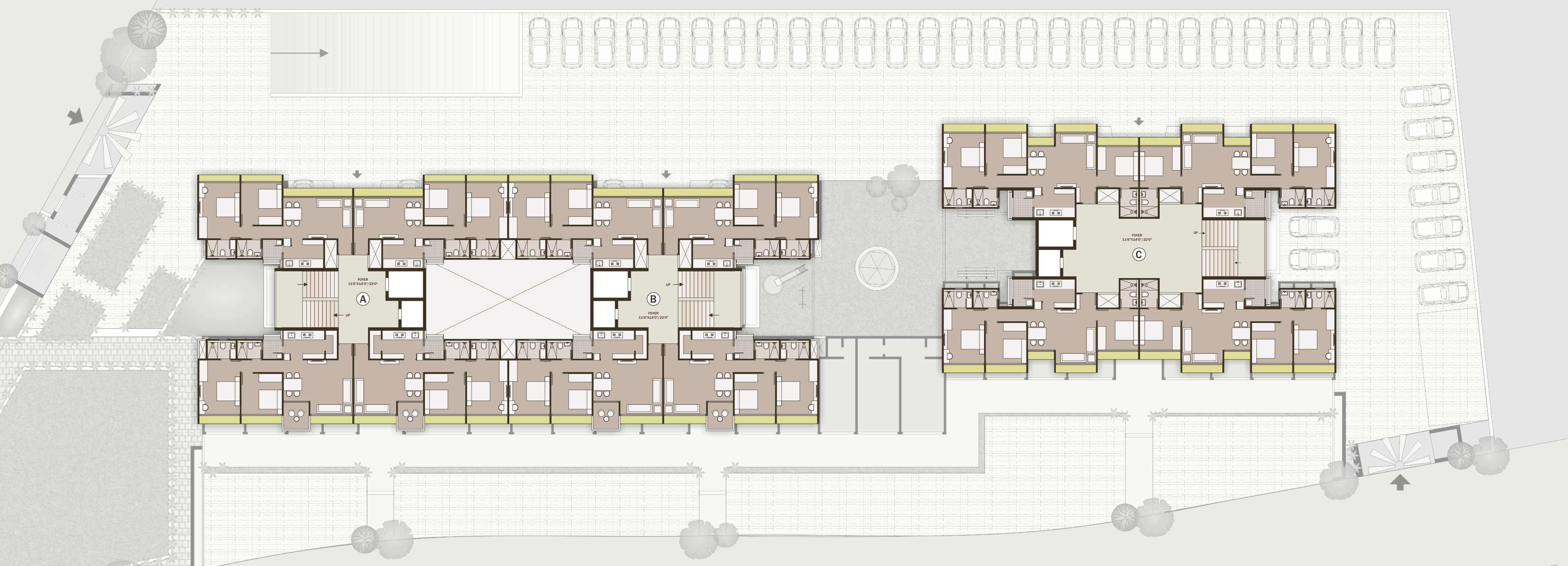
Typical Floor Plan
