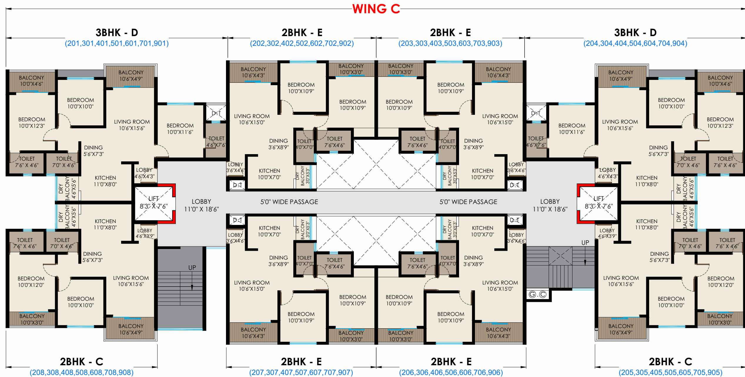
TYPICAL FLOOR - WING C
