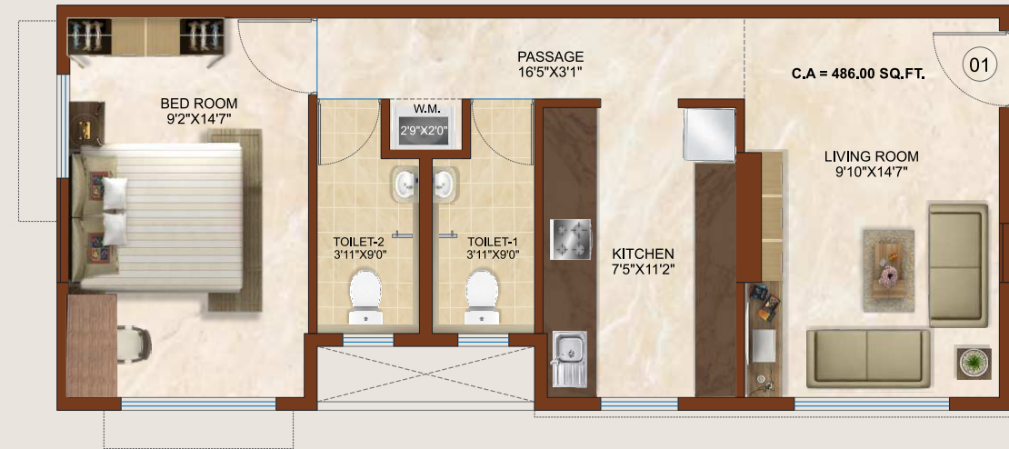
TYPICAL UNIT PLAN FLAT NO - 01 (1ST TO 4TH)
