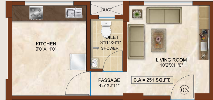
TYPICAL UNIT PLAN - OPTION 1 FLAT NO - 03 (1ST, 2ND & 4TH)
