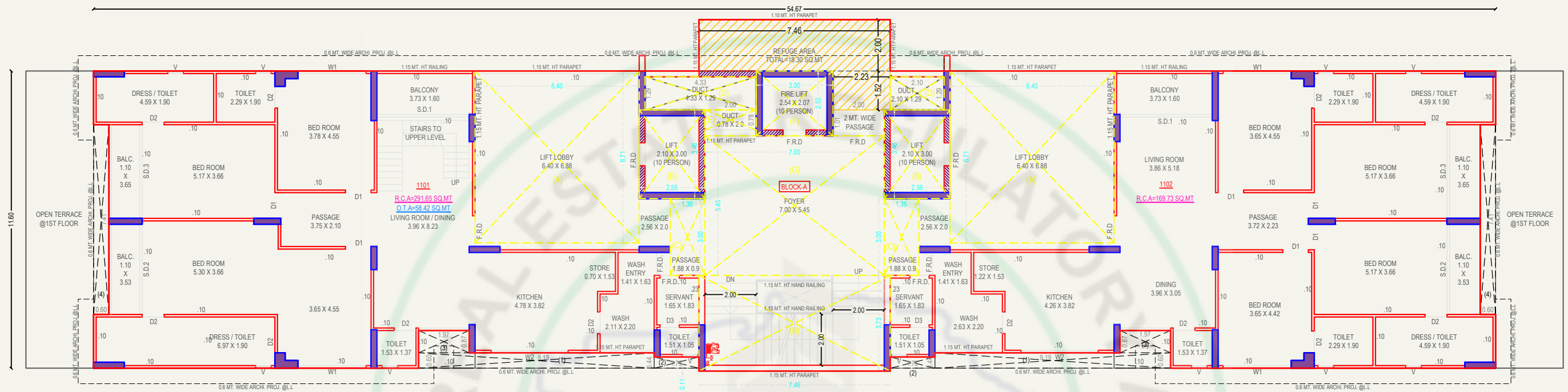
11TH FLOOR PLAN (BLOCK-A)
