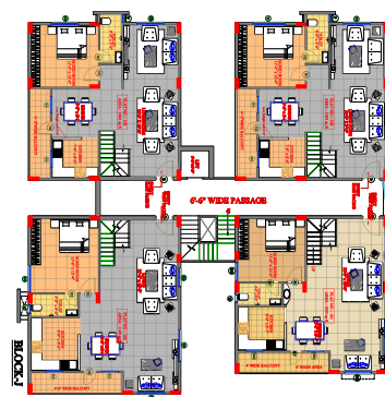
4BHK floor plan
