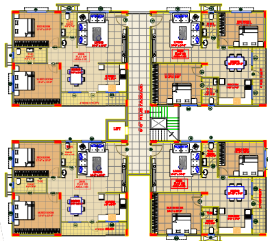
2BHK floor plan
