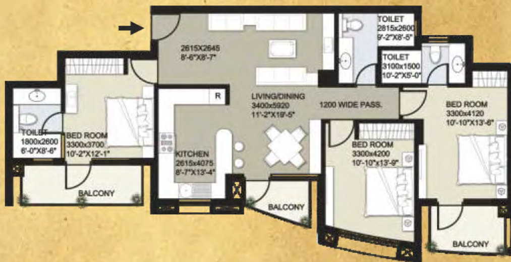
3BHK UNIT TYPE B Area:1795 sq. ft.
