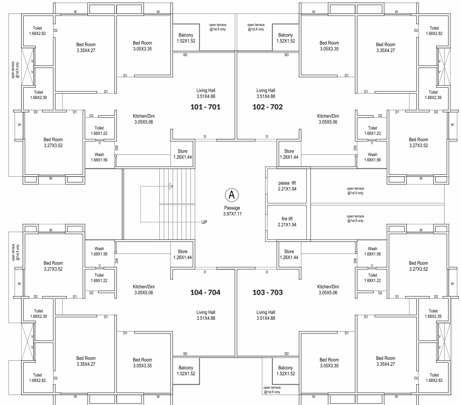
TOWER A & C 3 BHK Typical Floor Plan (1st - 7th Floor)
