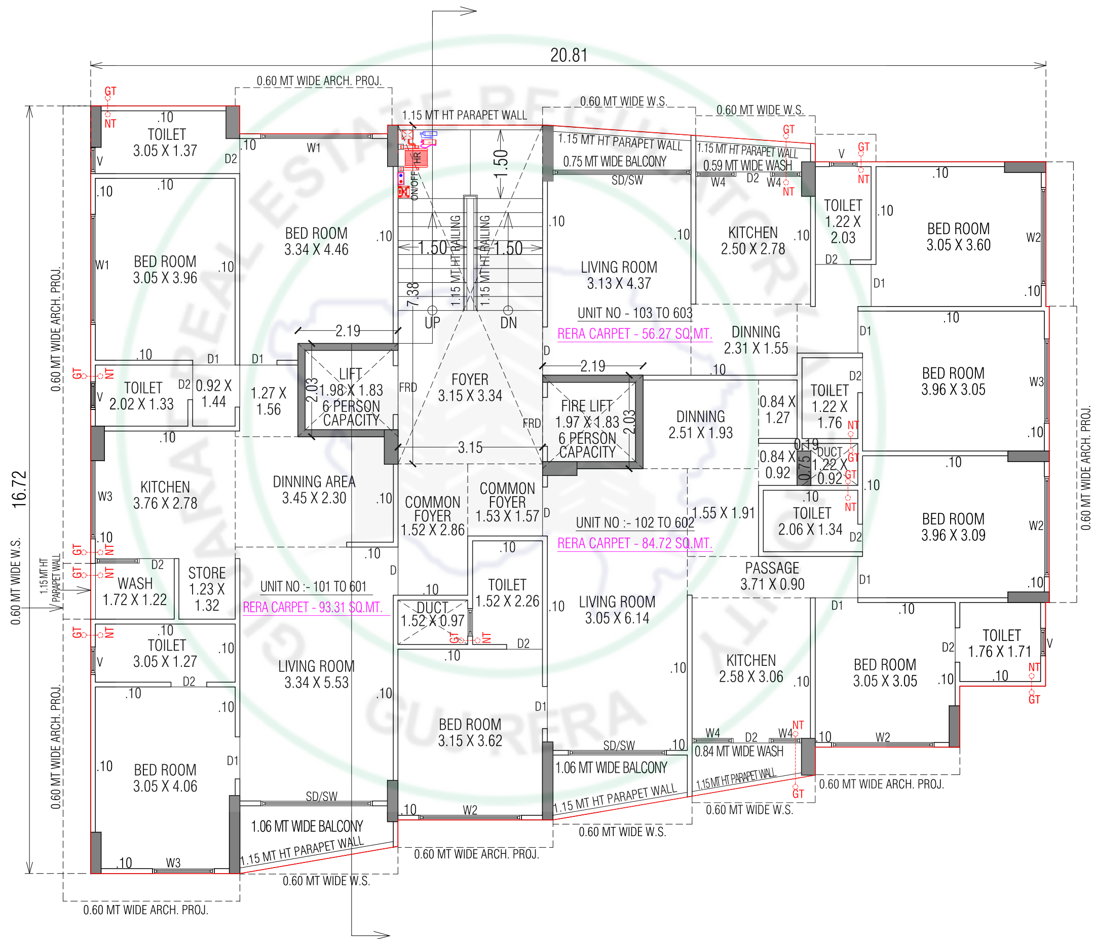
TYPICAL FLOOR PLAN (1ST TO 6TH)
