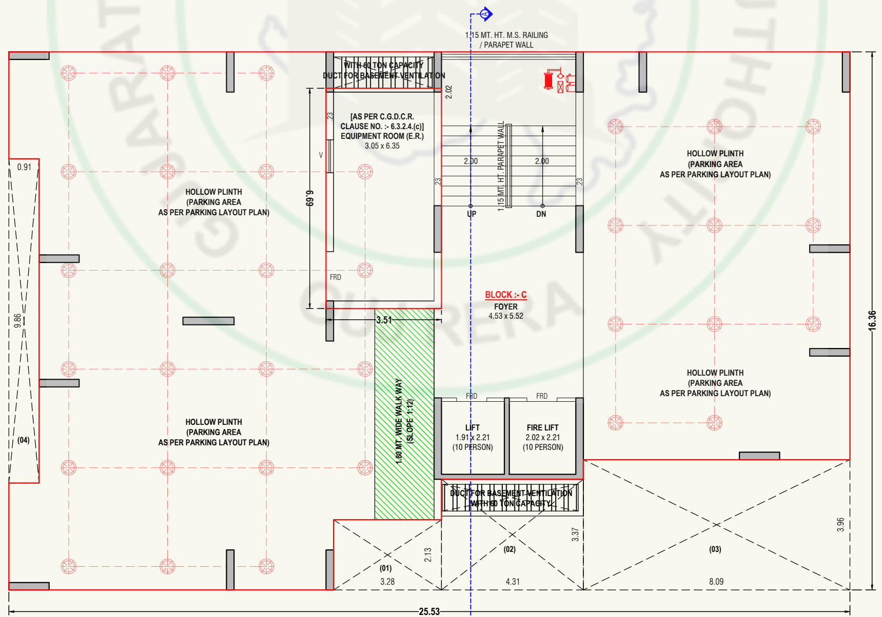
GROUND FLOOR PLAN (BLOCK-C)
