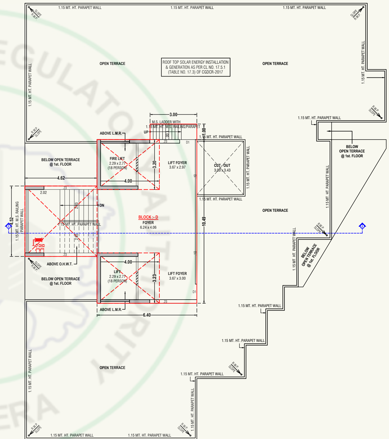
OPEN TERRACE PLAN WITH STAIR CABIN, LIFT MACHINE ROOM, O.H.W.T. (BLOCK-D)
