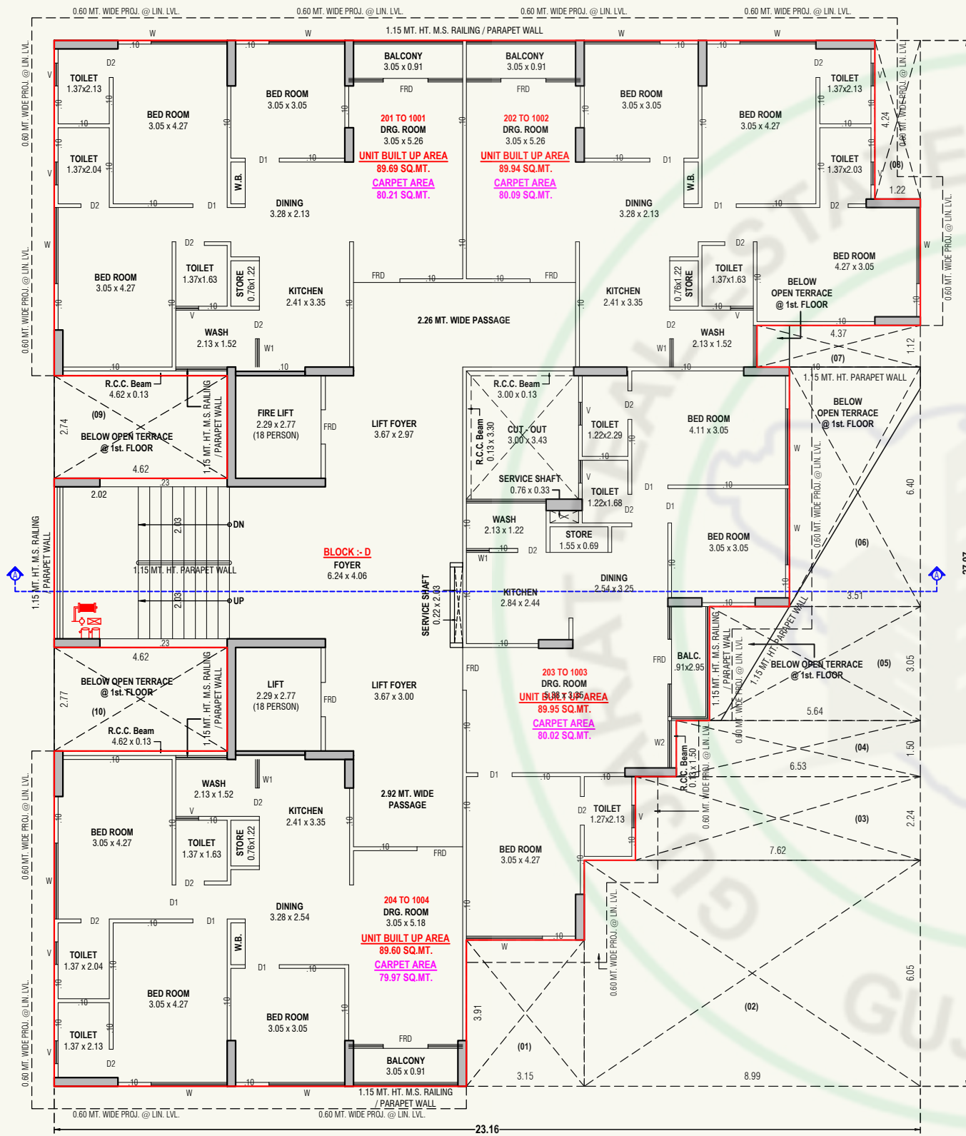
TYPICAL (2nd. to 10th.) FLOOR PLAN (BLOCK-D)
