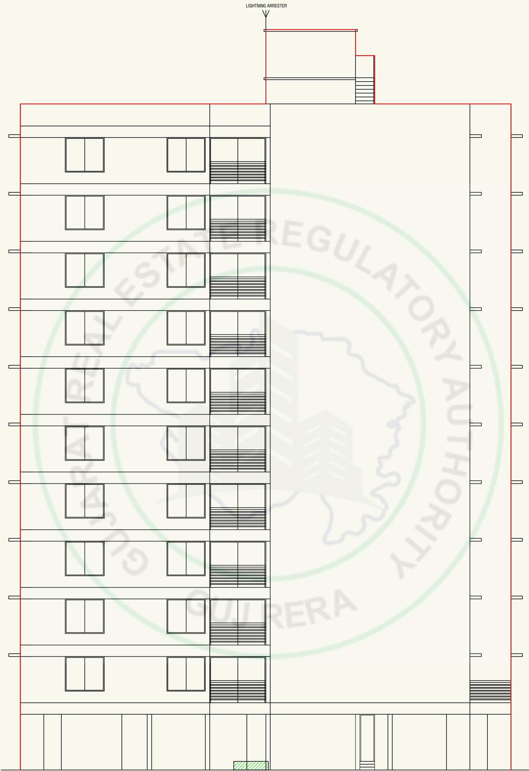
FRONT SIDE ELEVATION (BLOCK-C)
