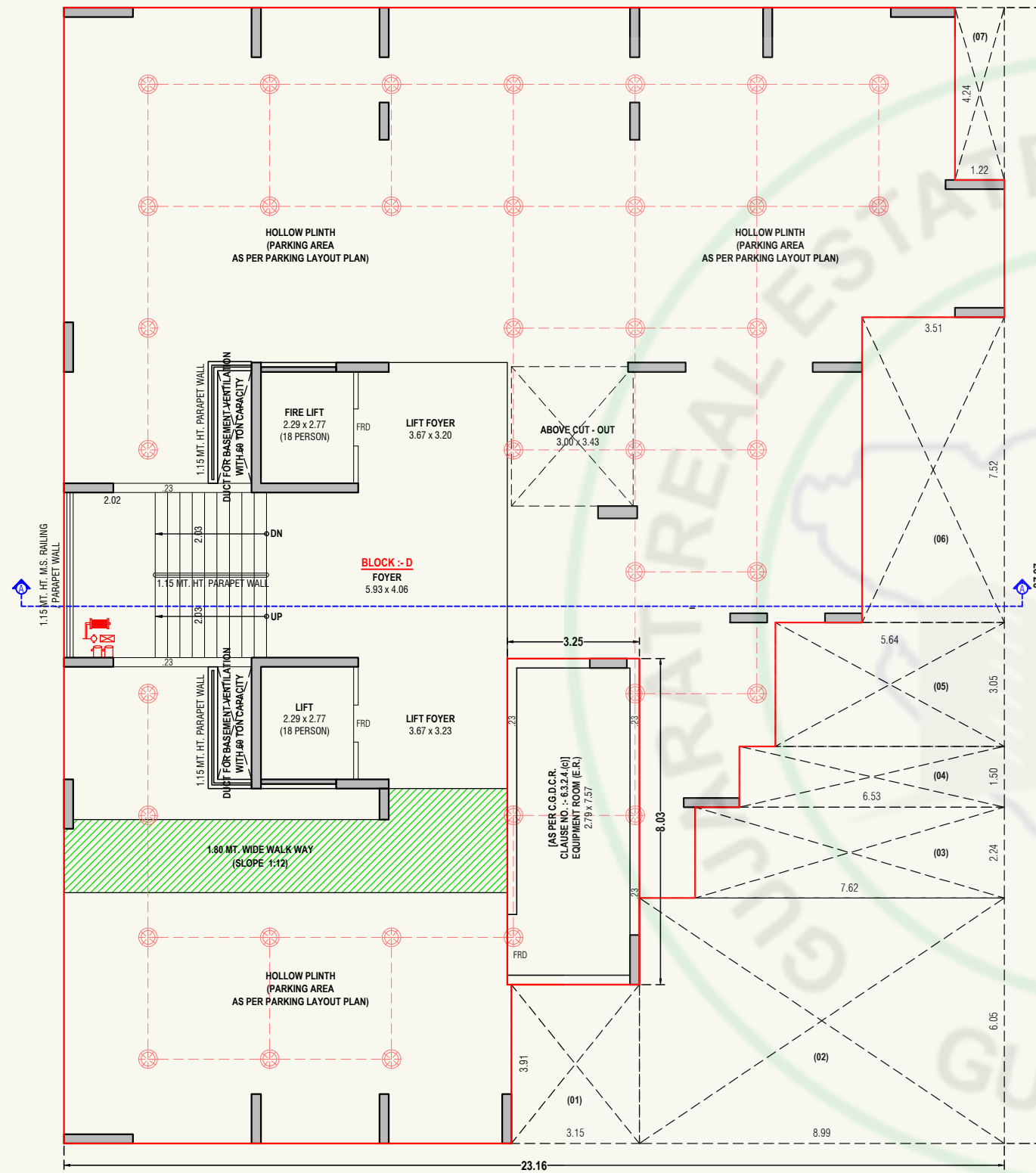
GROUND FLOOR PLAN (BLOCK-D)
