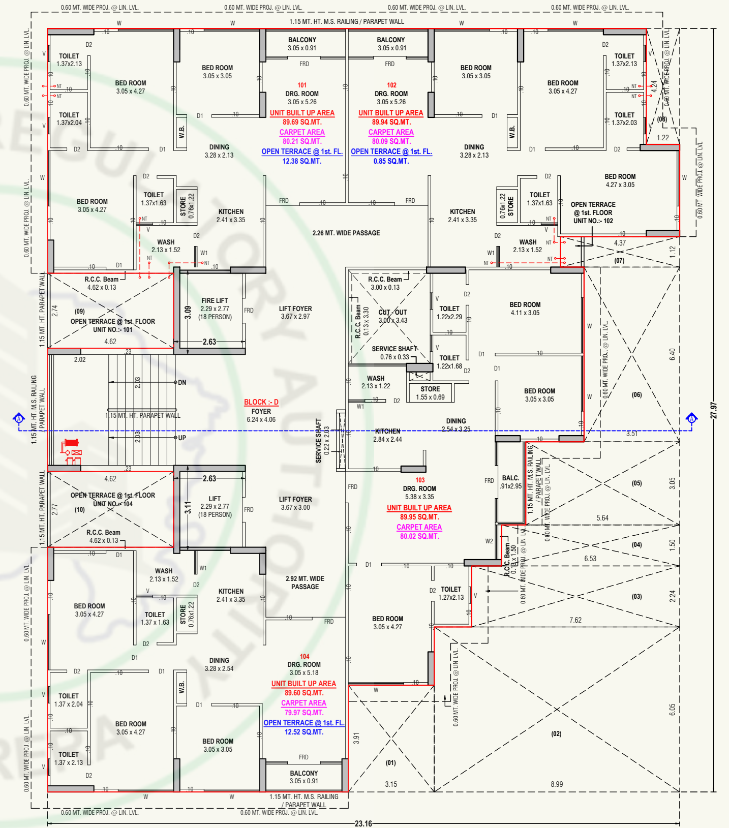
1st. FLOOR PLAN (BLOCK-D)
