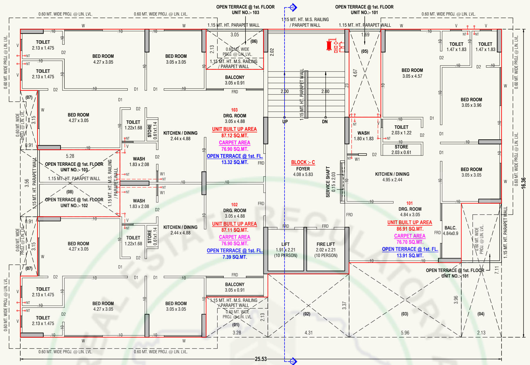
1st. FLOOR PLAN (BLOCK-C)
