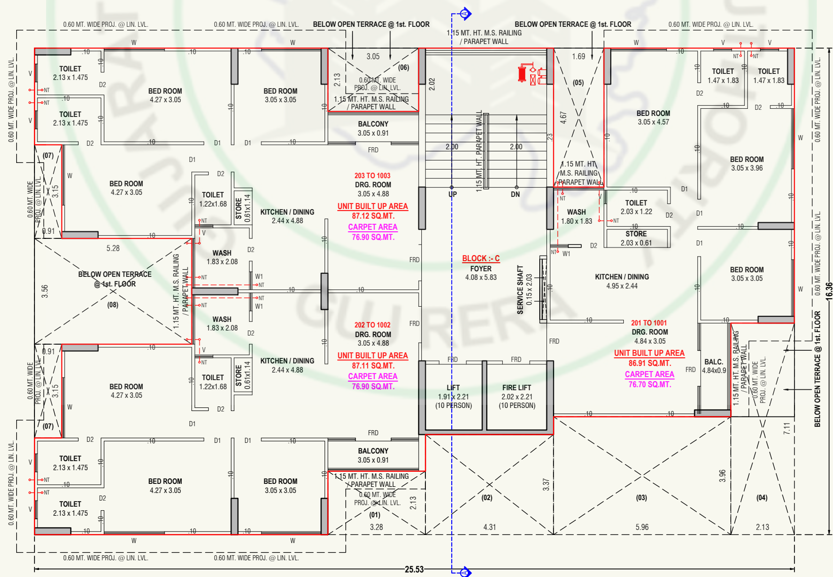
TYPICAL (2nd. to 10th.) FLOOR PLAN (BLOCK-C)
