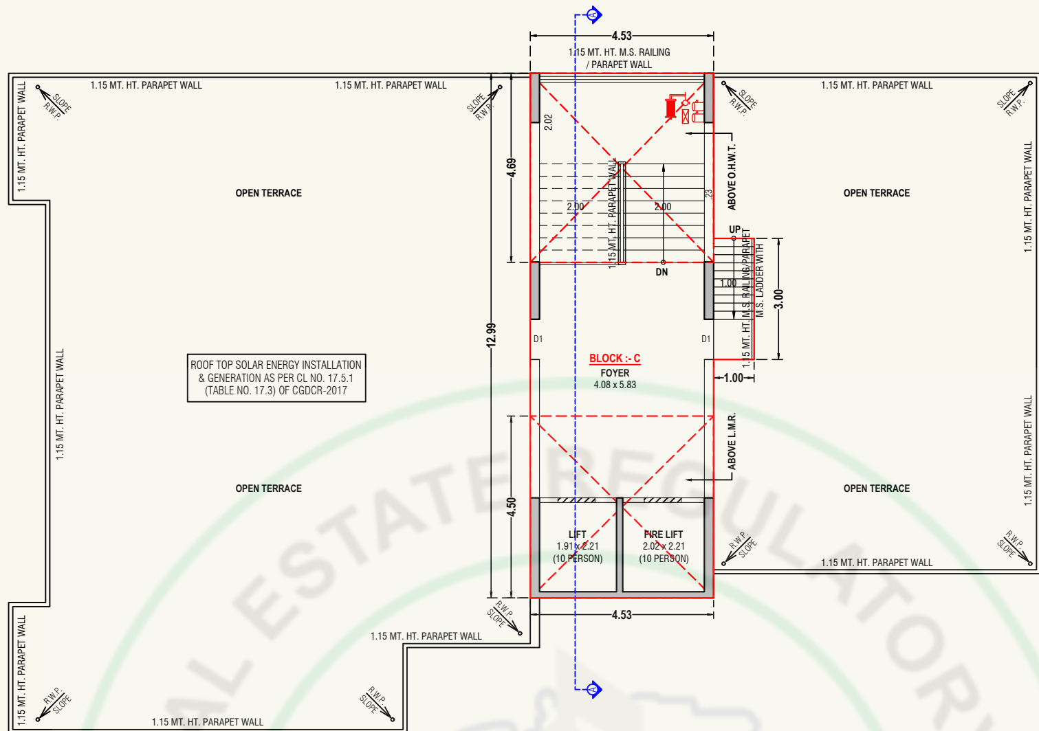
OPEN TERRACE PLAN WITH STAIR CABIN, LIFT MACHINE ROOM, O.H.W.T. (BLOCK-C)
