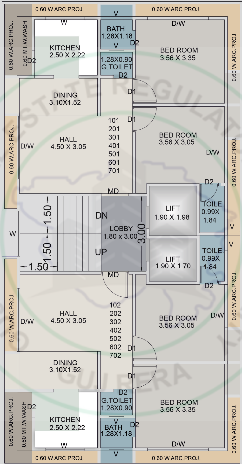
TYPICAL FLOOR
