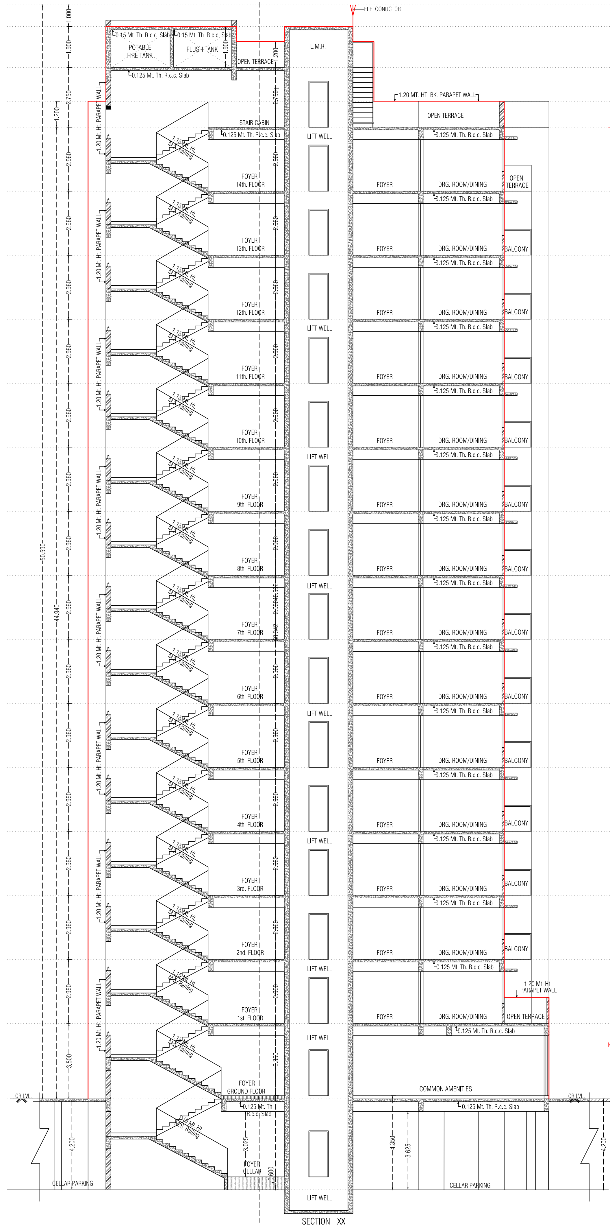
SECTION - XX
