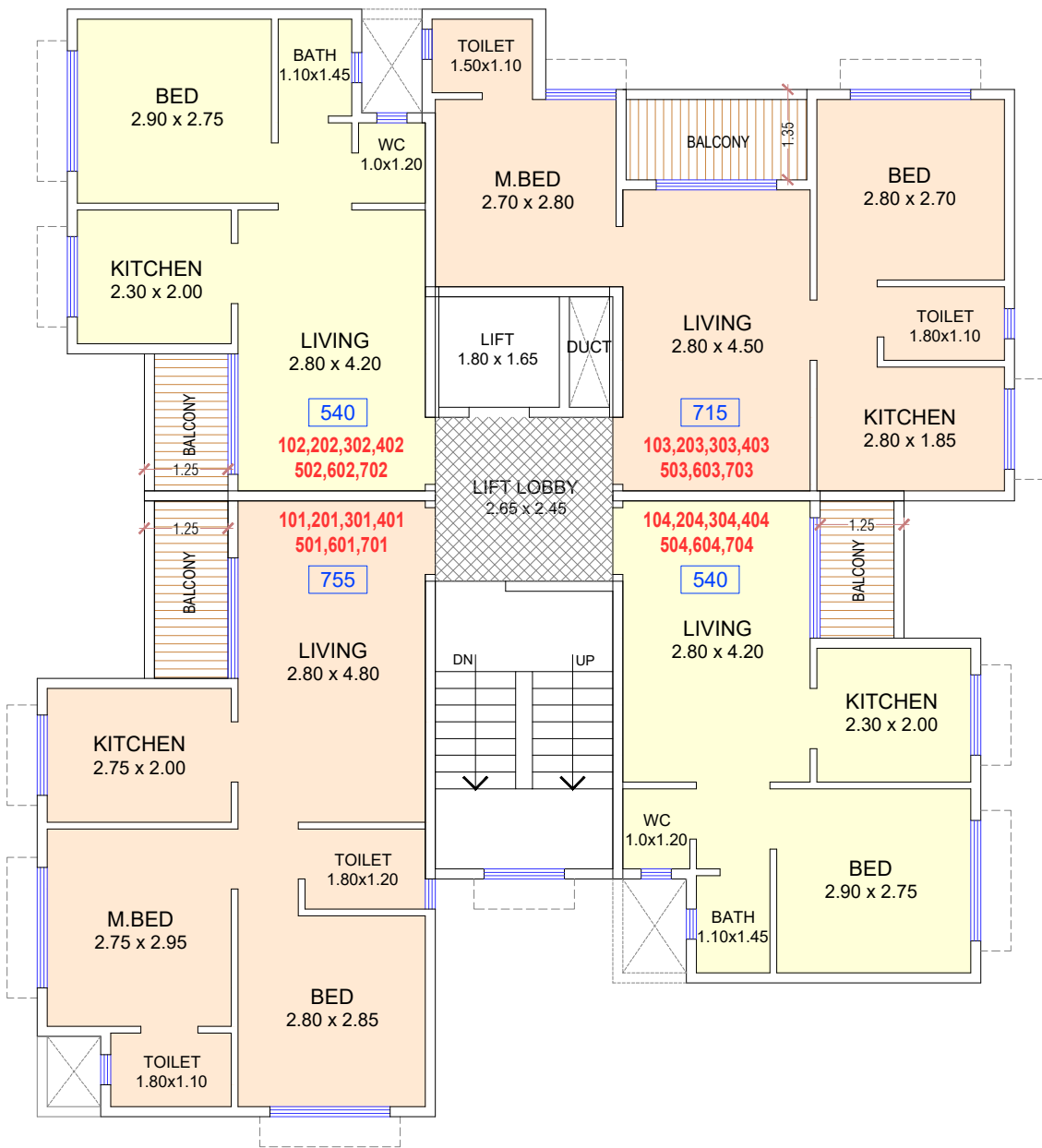
TYPICAL FLOOR PLAN (1st, 2nd, 3rd, 4th, 5th, 6th & 7th)
