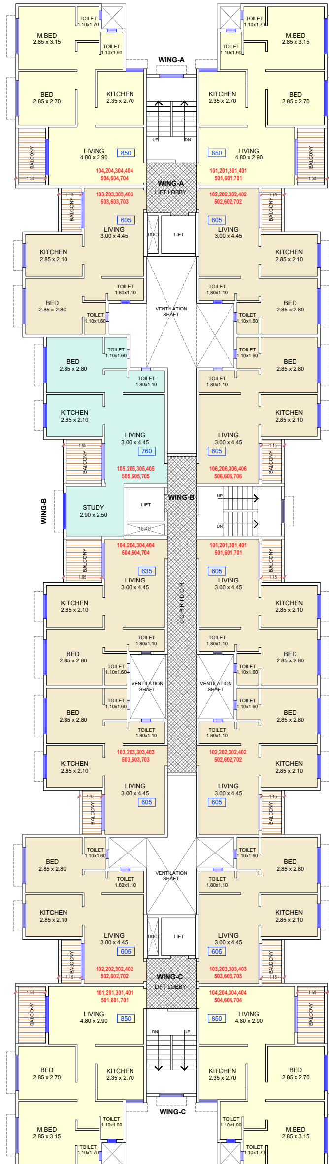
TYPICAL FLOOR PLAN (1st, 2nd, 3rd, 4th, 5th, 6th & 7th)
