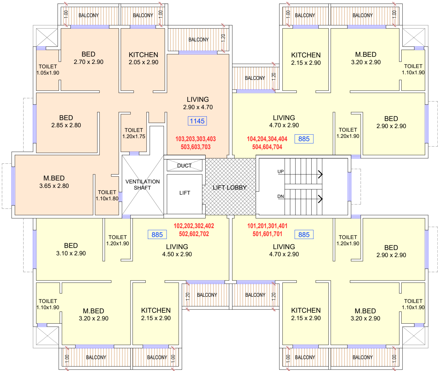
TYPICAL FLOOR PLAN (1st, 2nd, 3rd, 4th, 5th, 6th & 7th)
