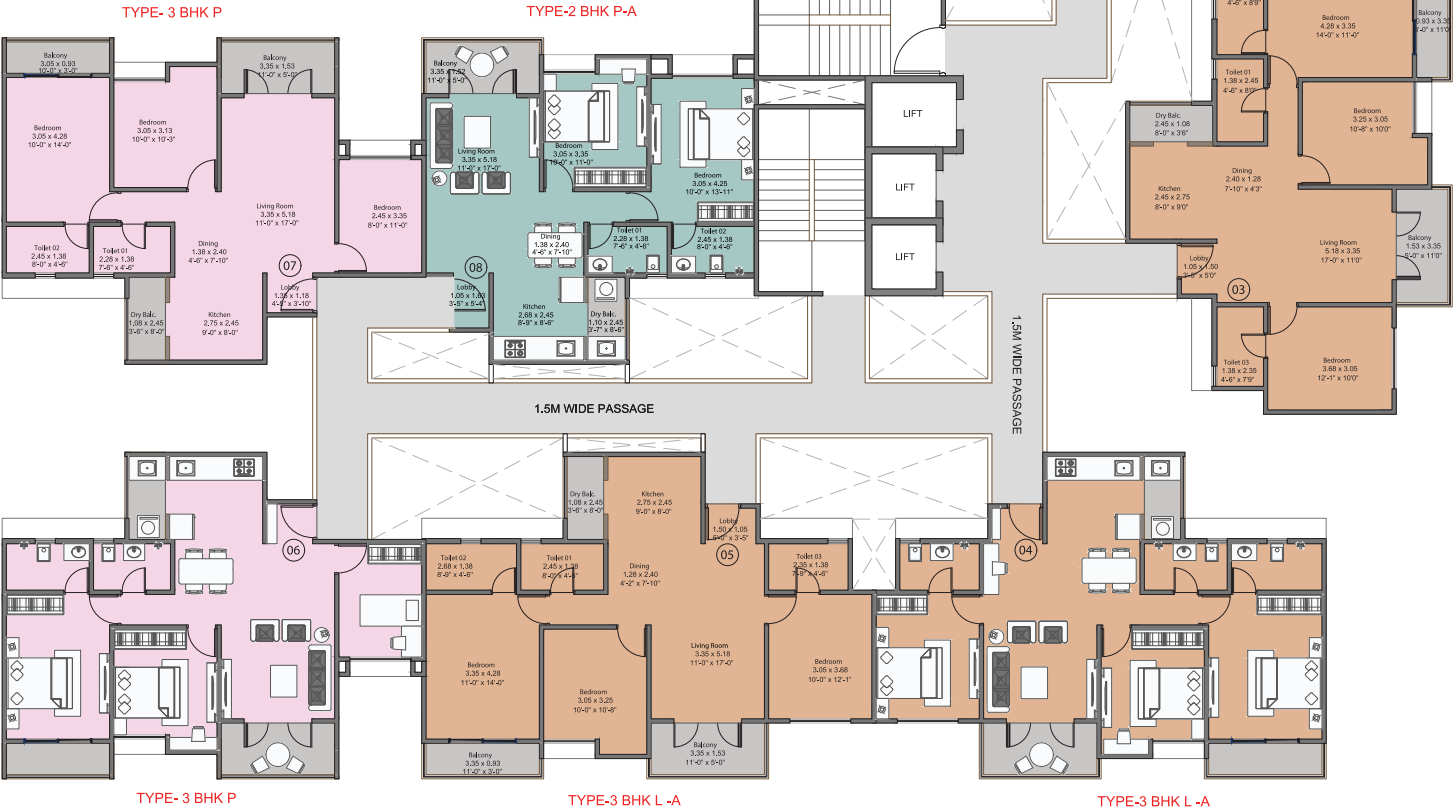
1 ST , 2 ND , 3 RD , 4 TH , 5 TH , 6 TH , 7 TH , 9 TH , 10 TH , 11 TH , 12 TH , 14 TH & 15 TH FLOOR PLAN
