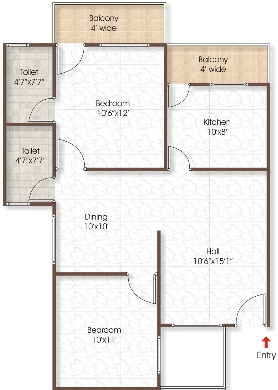
2 BHK Type-1 S.B.A. - 990.41 Sq. Ft.
