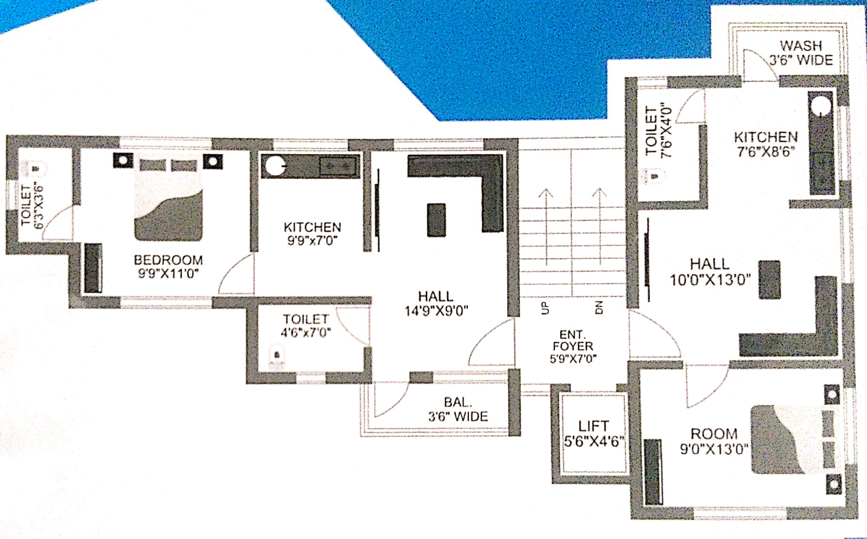
TYPICAL FLOOR (1,2,3,4th)
