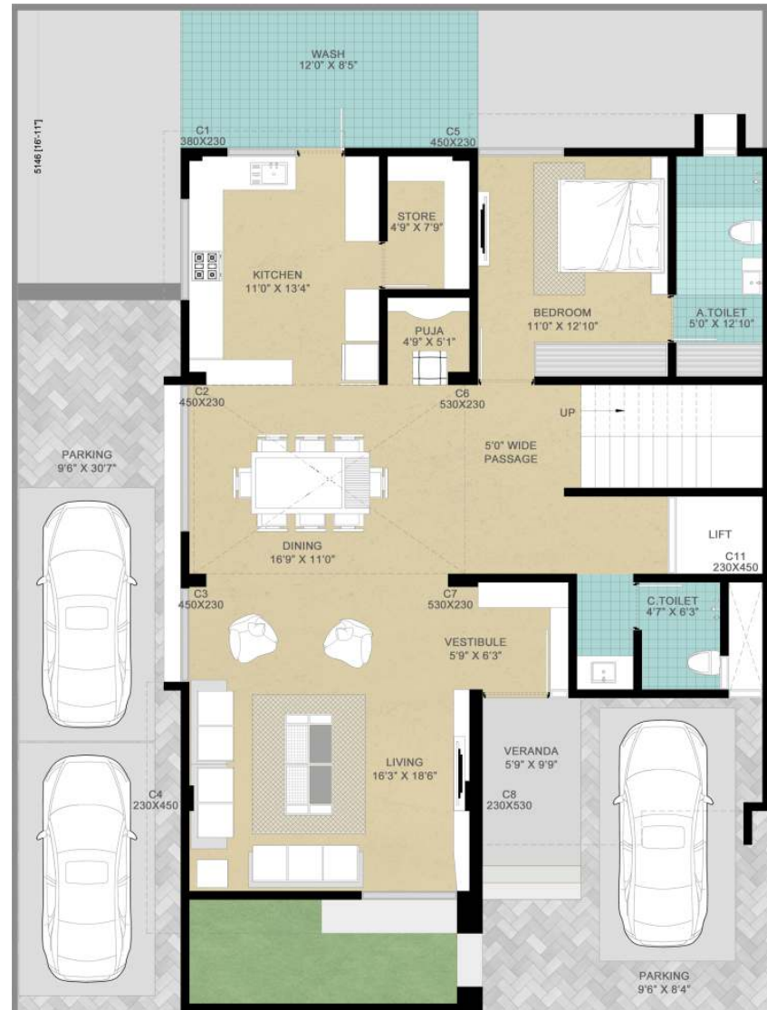
Ground Floor
