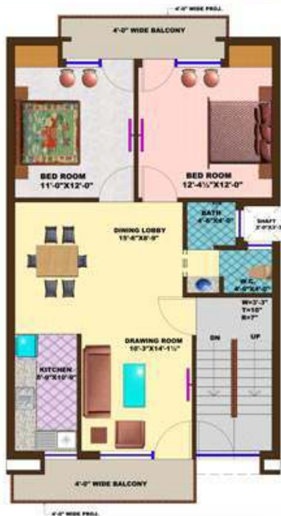
Typical Floor Plan Plot Area = 150 sq. yd (Approx) Super Built-up Area = 1050 sq. ft.
