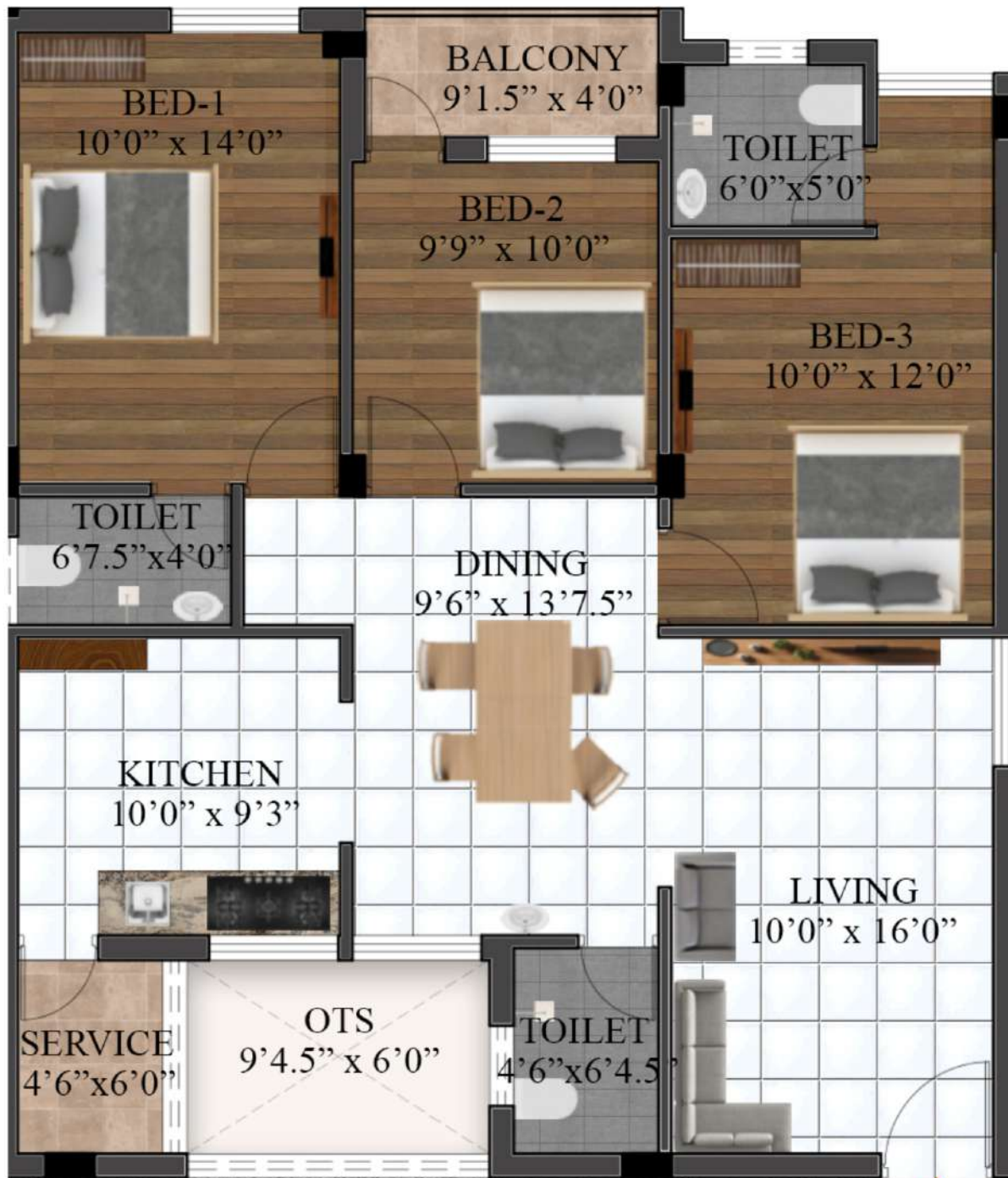
GROUND, FIRST & SECOND FLOOR PLAN
