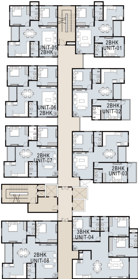
TYPICAL FLOOR PLAN NOT TO SCALE
