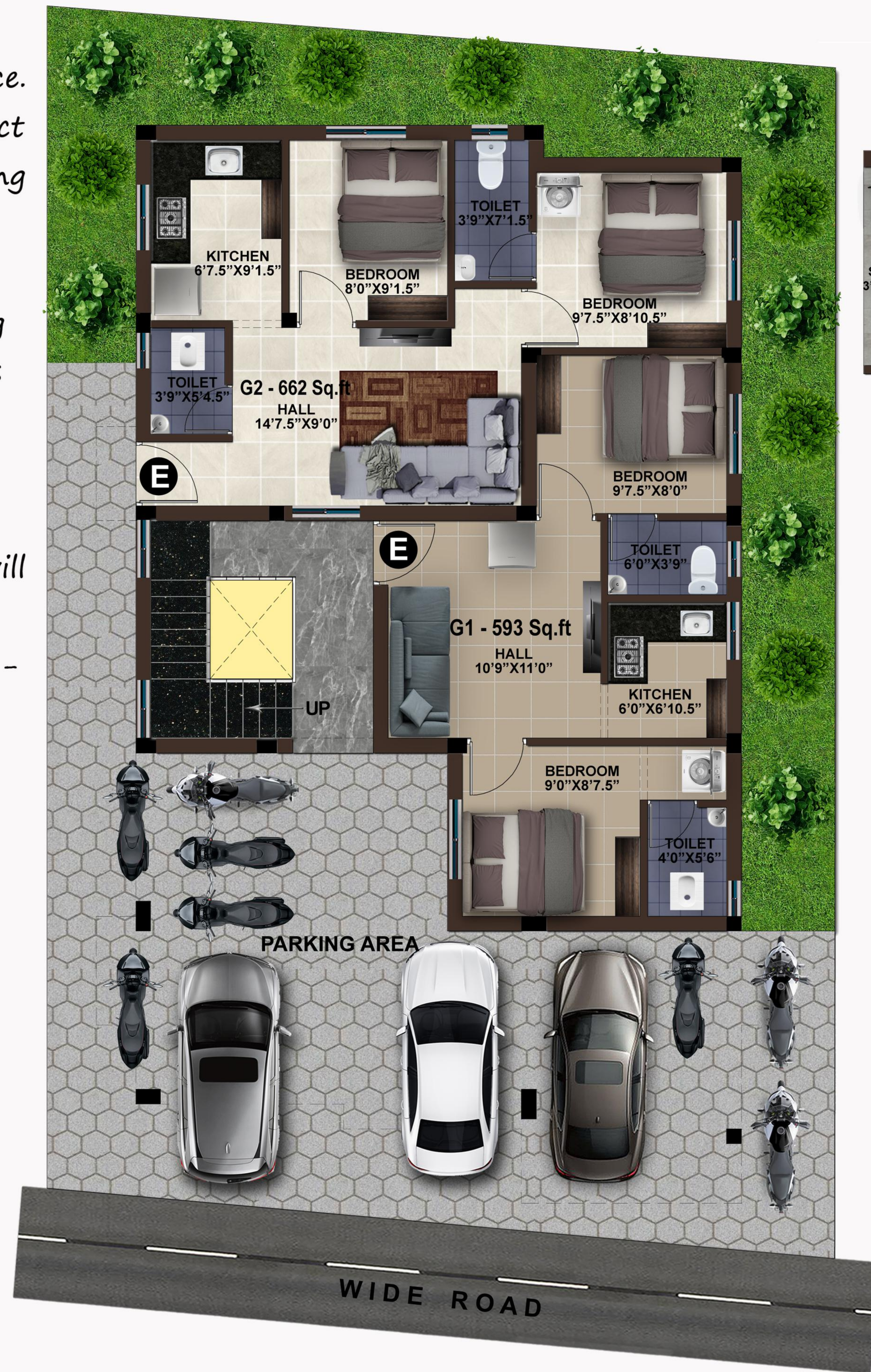
GROUND FLOOR
