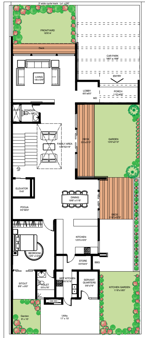
Ground Floor (Builtup Area: 1847 sft )
