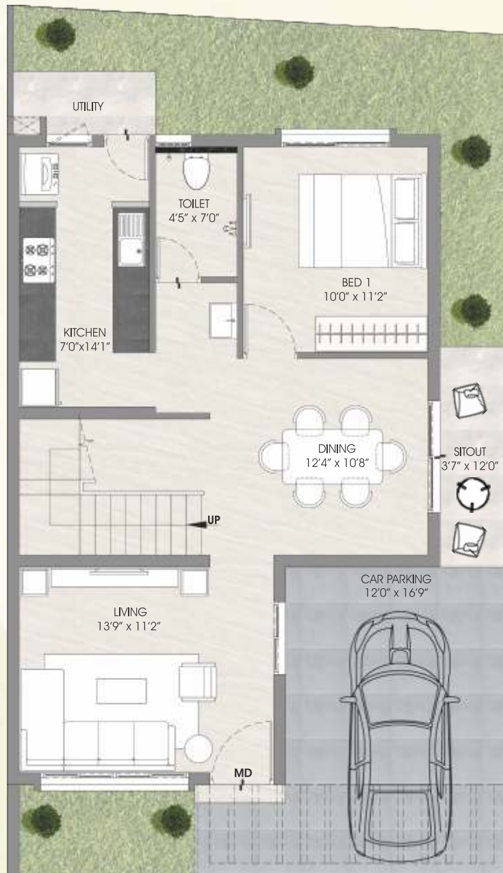
Ground Floor
