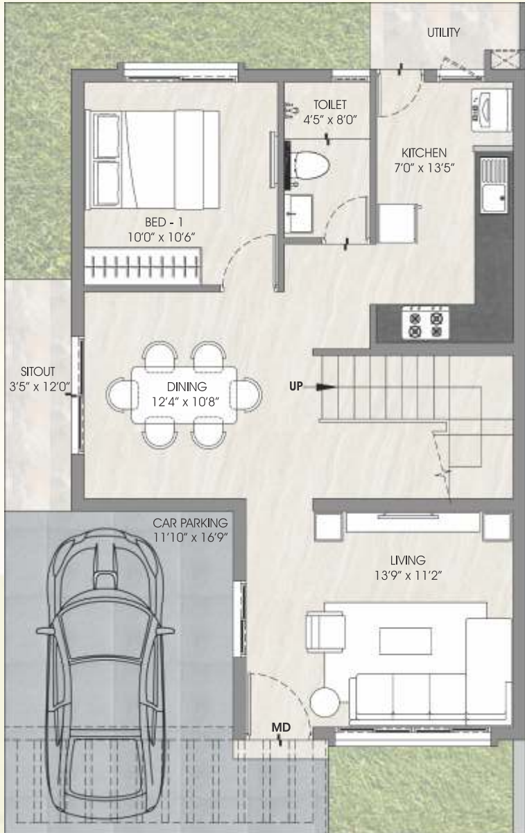
Ground Floor
