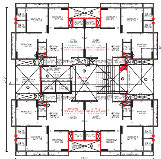
TYPICAL FLOOR PLAN (2ND. TO 13TH. FLOOR PLAN)
