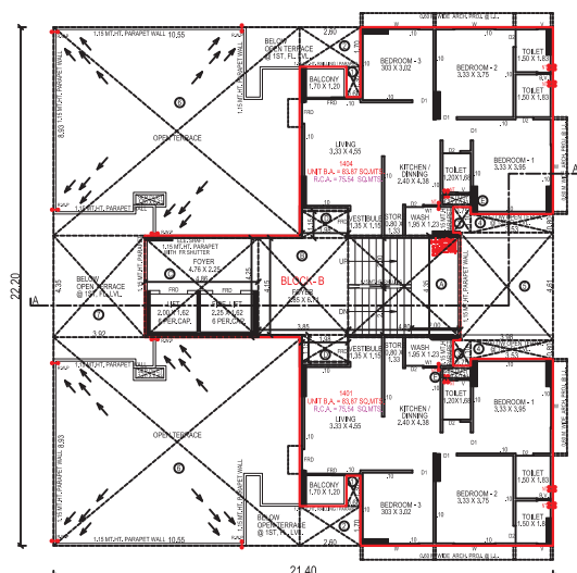
14TH. FLOOR PLAN
