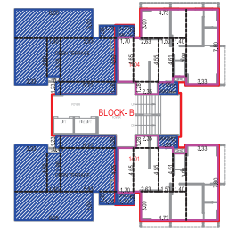
BERA CARPET AREA CALCULATION (14TH. FLOOR PLAN)
