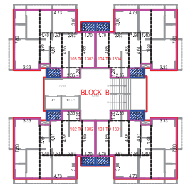
BERA CARPET AREA CALCULATION (1ST. TO 13TH. FLOOR PLAN)
