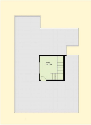
Terrace Plan
