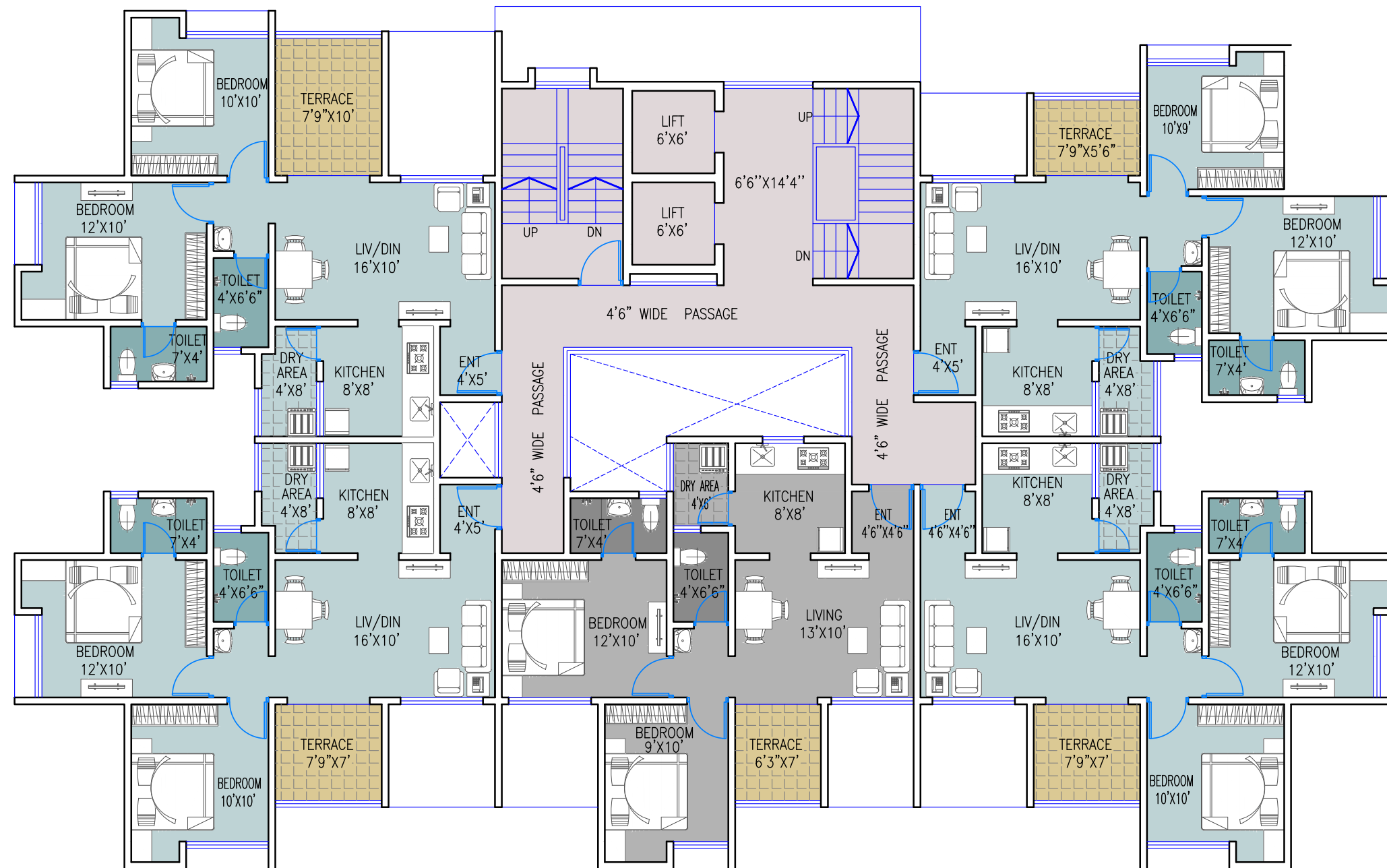
TYPICAL 2ND, 4TH, 6TH & 8TH FLOOR PLAN
