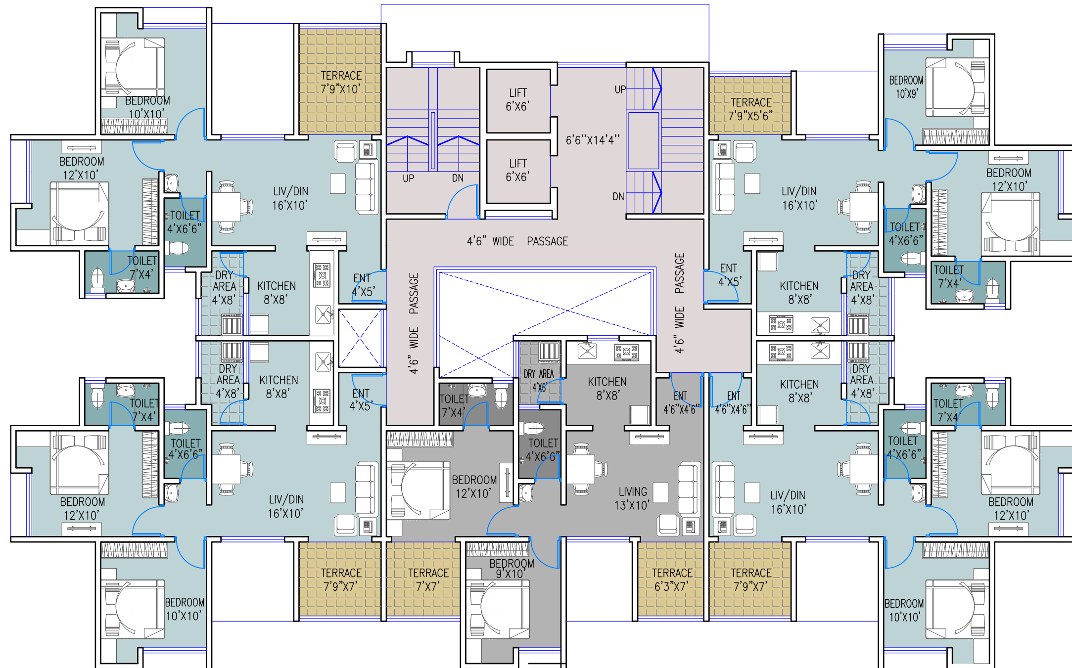
TYPICAL 1ST, 3RD, 5TH AND 7TH FLOOR PLAN
