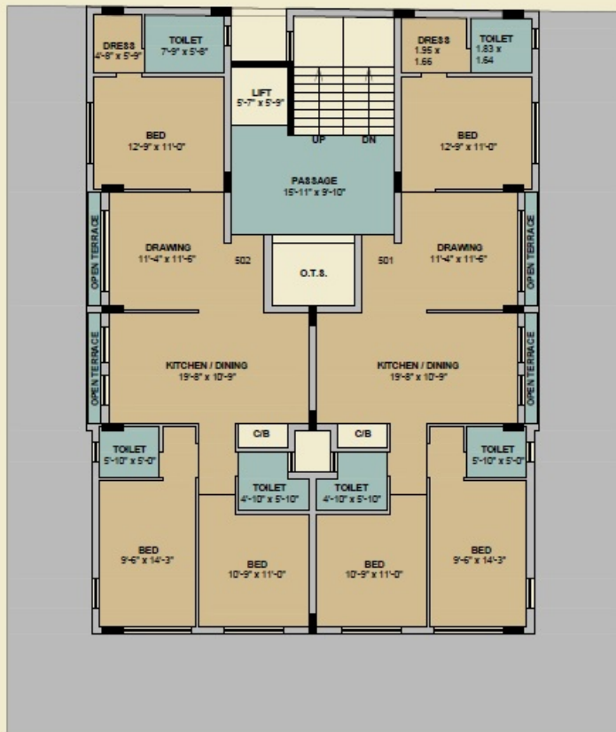
5th FLOOR PLAN
