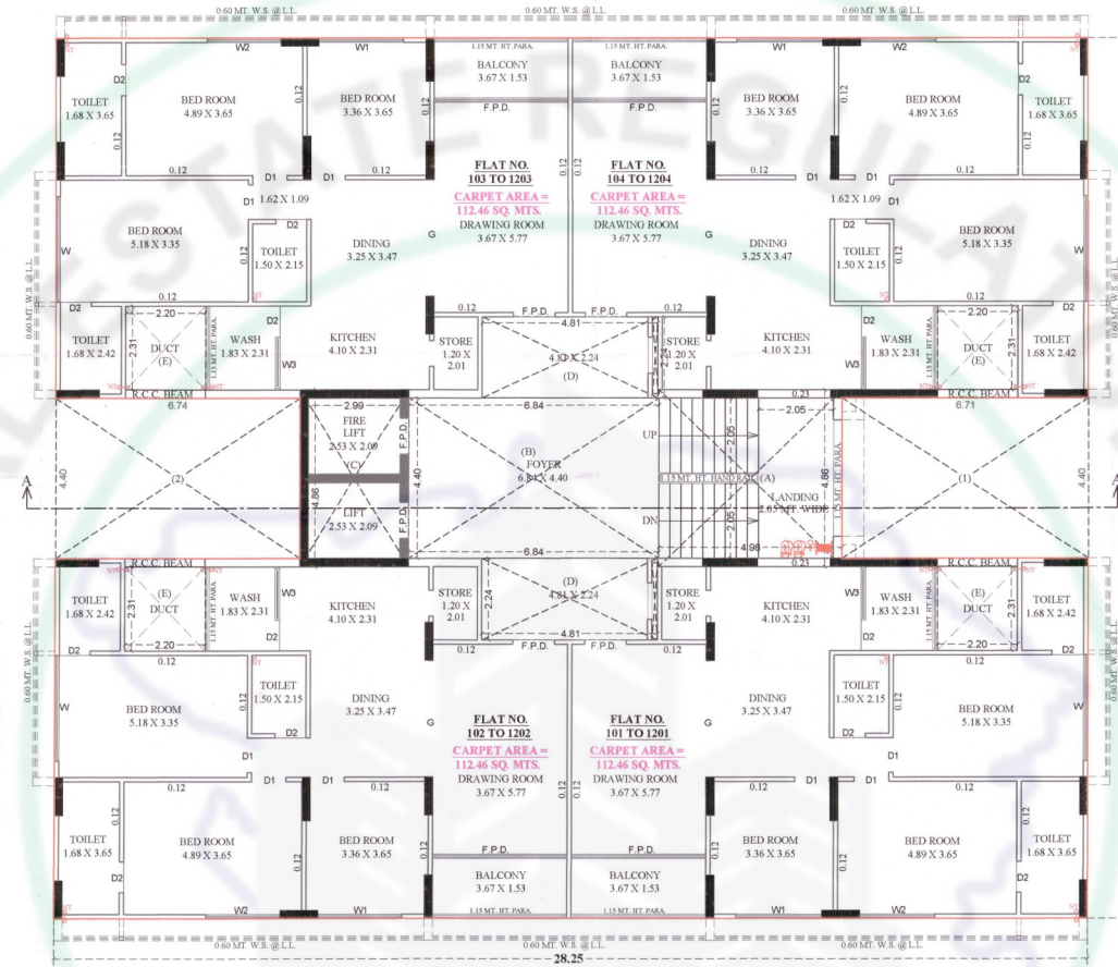
TYPICAL FLOOR
