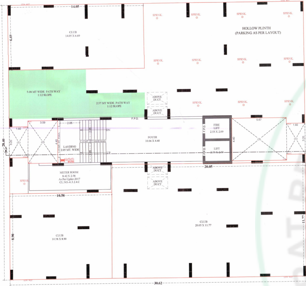
GROUND FLOOR
