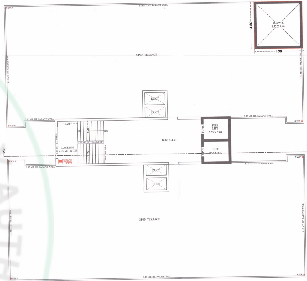
TERRACE FLOOR
