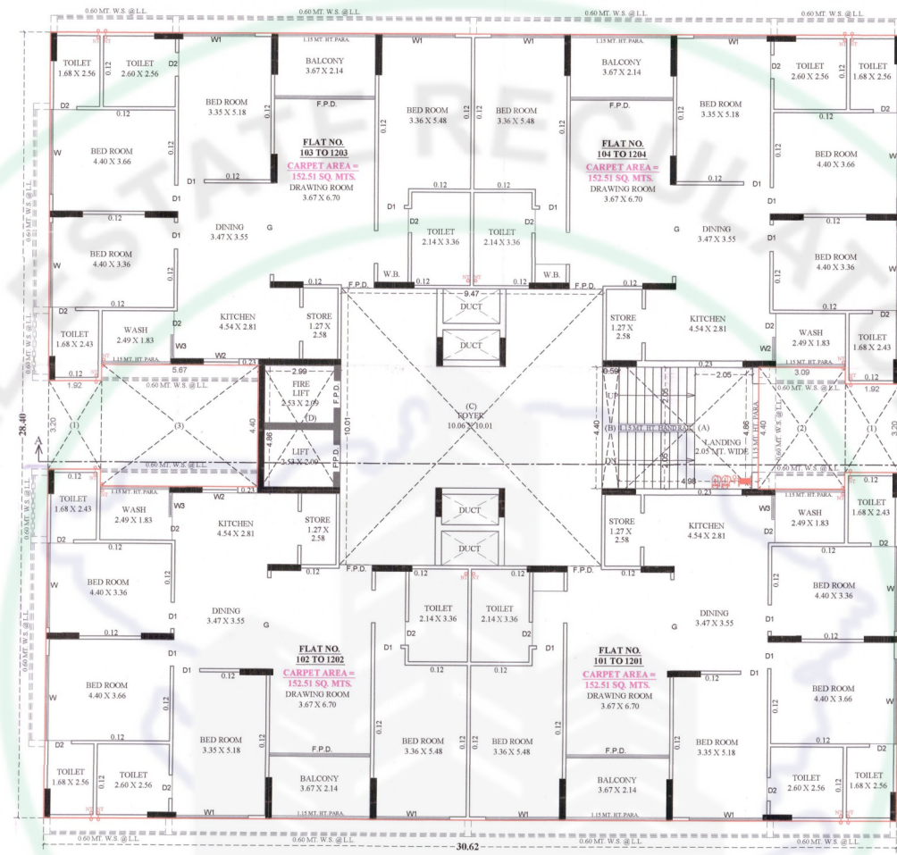
TYPICAL FLOOR
