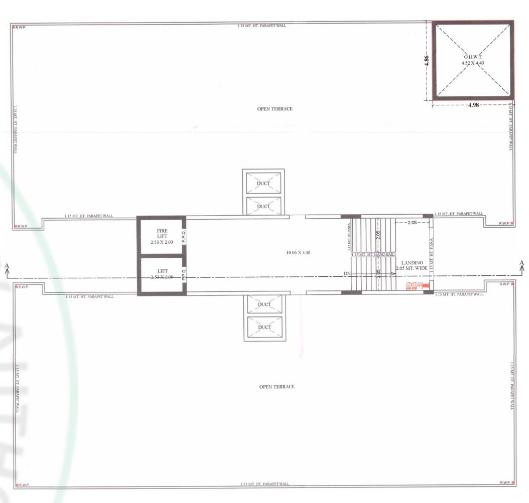
TERRACE FLOOR
