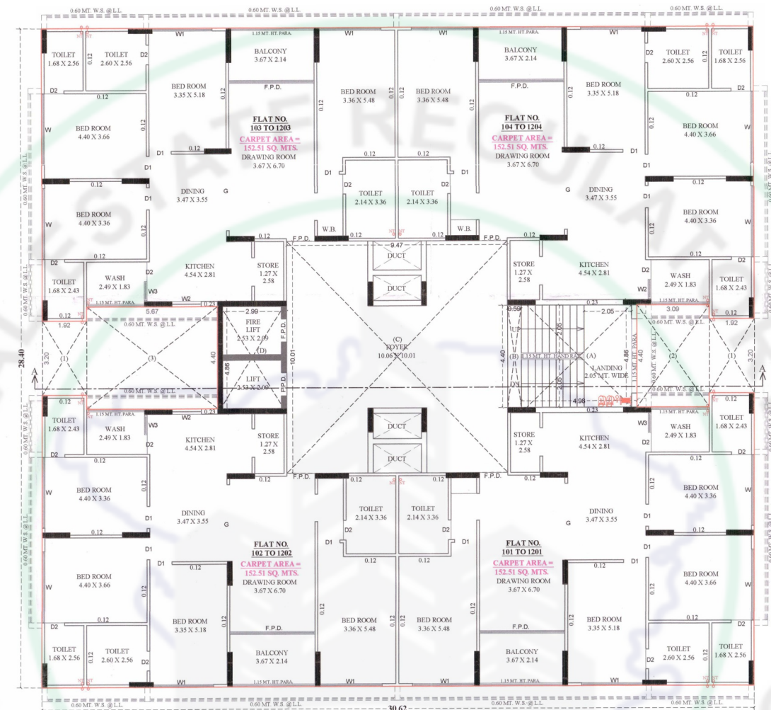
TYPICAL FLOOR
