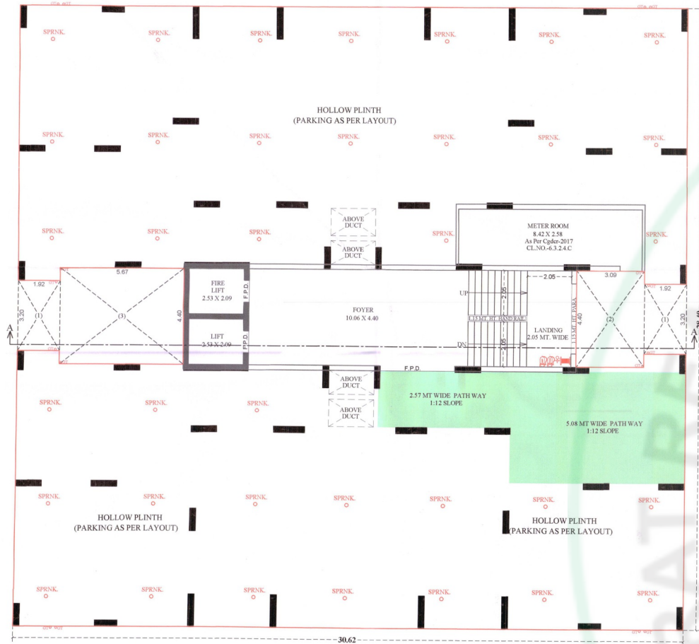
GROUND FLOOR
