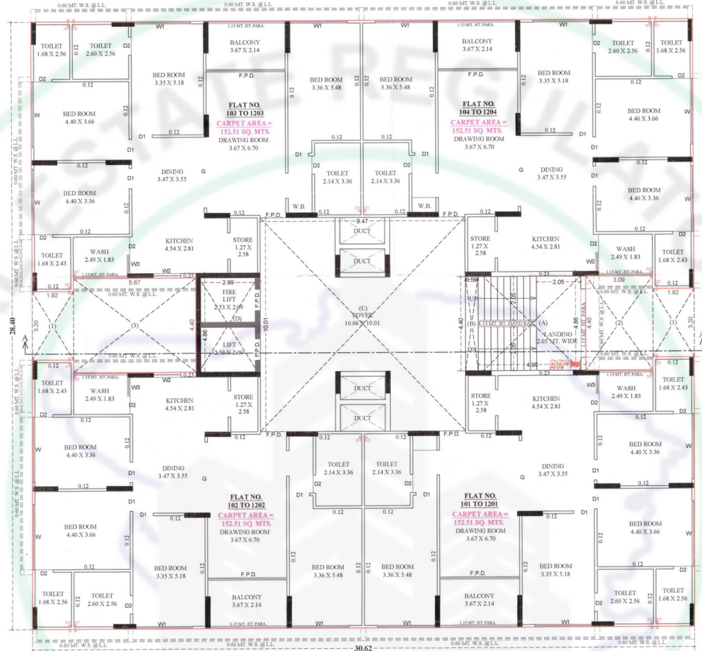
TYPICAL FLOOR
